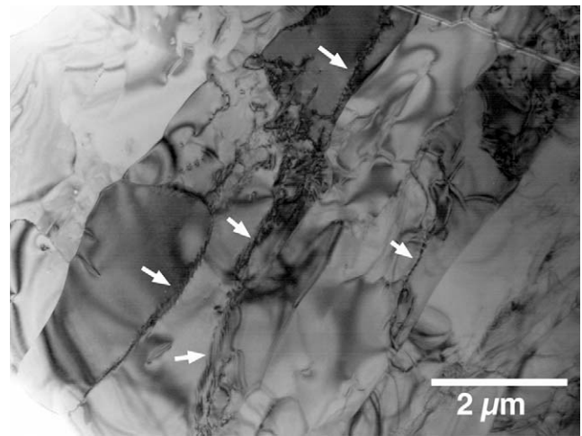
Fig. 10. Bright-field TEM image of a majorite crystal in a polycrystalline aggregate from Sixiangkou. The majorite crystals are >10 \mu\text{m} in size and contain numerous subgrain boundaries.
