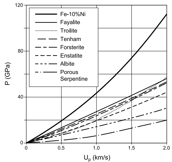
Fig. A-1. P- U_p Hugoniots of some chondritic minerals and a synthetic Hugoniot for Tenham.
