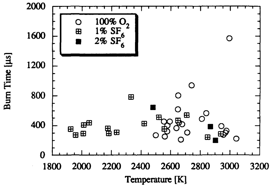
Figure 4.33 Burn time versus temperature of the third peak comparing SF 6 and O 2 for 20 μm boron particles at 125 psia.
