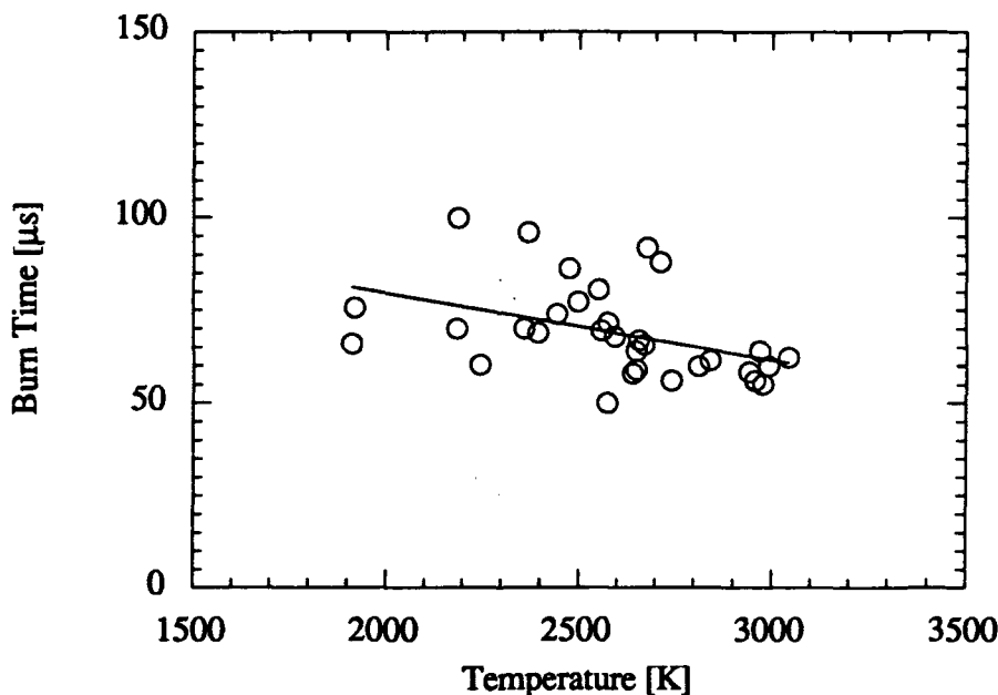
Figure 4.12 Burn time versus temperature of the first two peaks in 100% oxygen atmosphere at 125 psia for 20\ \mu\text{m} crystalline boron particles. The line represents a linear curve fit to the data.
