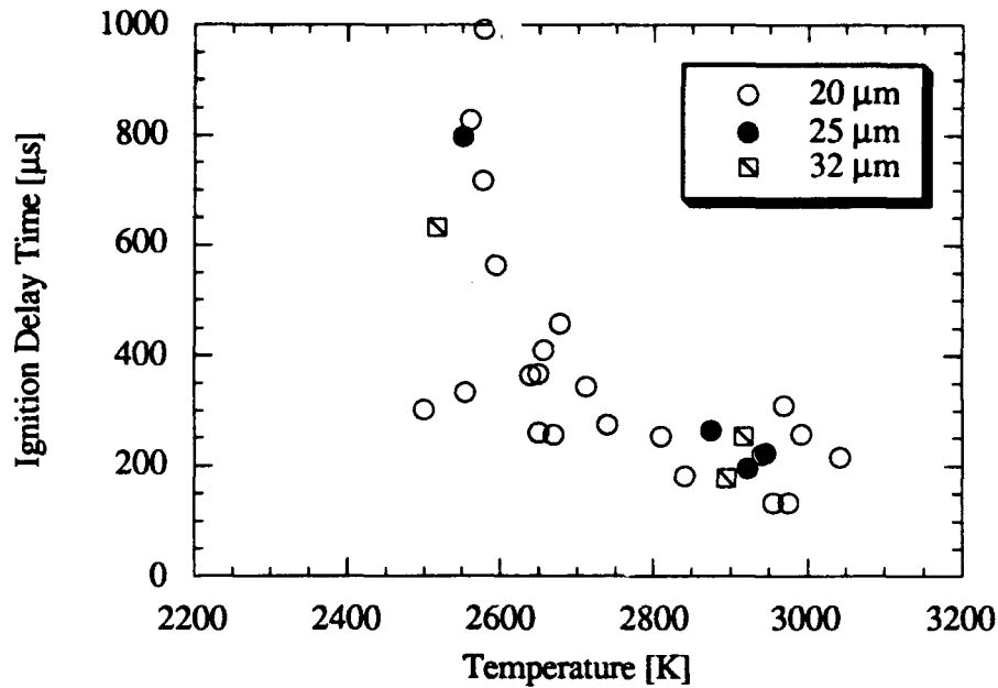
Figure 4.20 Ignition delay time versus temperature of the third peak in 100% oxygen atmosphere at 125 psia for 20, 25, and 32 \mu\text{m} crystalline boron particles.
