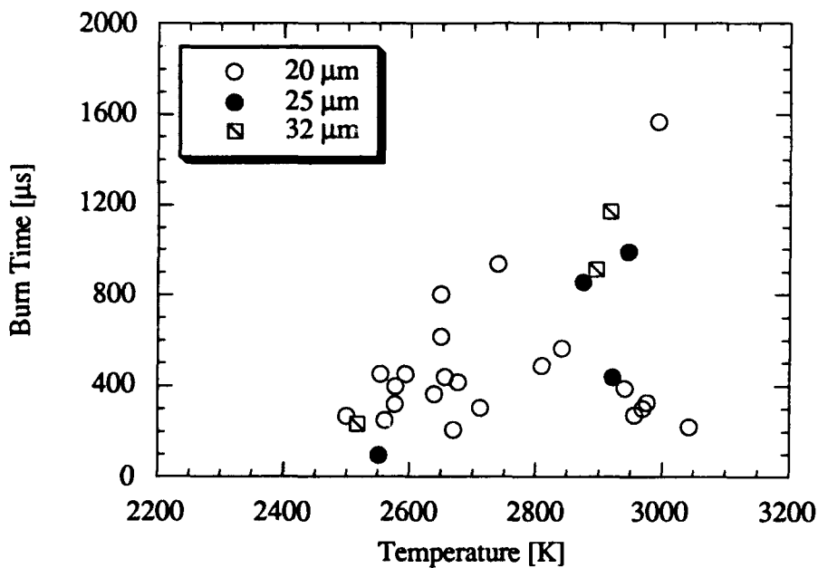
Figure 4.21 Burn time versus temperature of the third peak in 100% oxygen atmosphere at 125 psia for 20, 25, and 32 \mu\text{m} crystalline boron particles.
