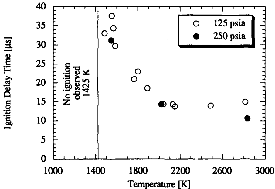
Figure 4.6 Amorphous boron ignition delay time versus temperature at two pressures. All conditions tested with 100% oxygen. The ignition limit of 1425 K is found at 125 psia.
