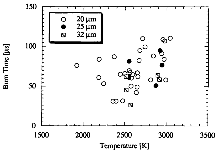
Figure 4.19 Burn time versus temperature of the first two peaks in 100% oxygen atmosphere at 125 psia for 20, 25, and 32 \mu\text{m} crystalline boron particles.
