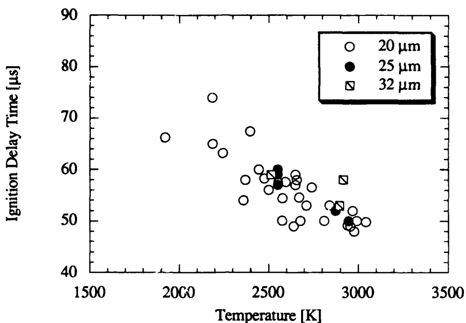
Figure 4.18 Ignition delay time versus temperature for the first peak in 100% oxygen atmosphere at 125 psia for 20, 25, and 32 \mu\text{m} crystalline boron particles.
