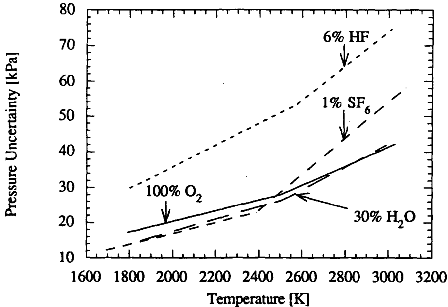
Figure 4.36 Pressure uncertainty as a function of temperature and oxidizer mixture at a test pressure of 860 kPa (125 psia). The partial mole fraction gases are complemented with oxygen.
