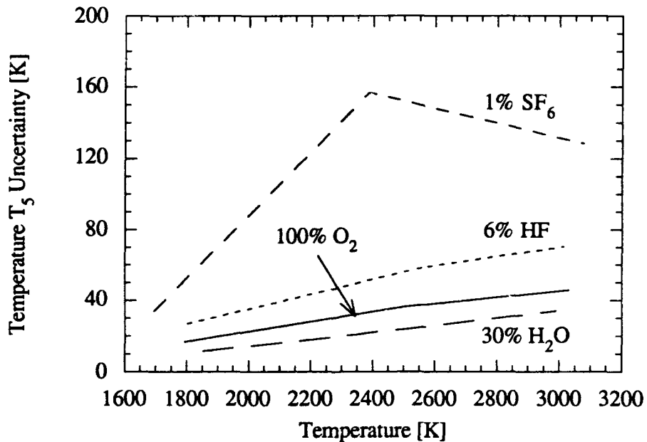
Figure 4.36 Temperature T_5 uncertainty as a function of temperature and oxidizer mixture at a test pressure of 860 kPa (125 psia). The partial mole fraction gases are complemented with oxygen.
