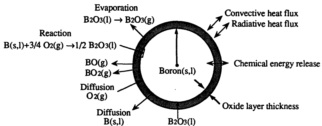
Figure 1.1 Classical ignition model of boron particle [1].
