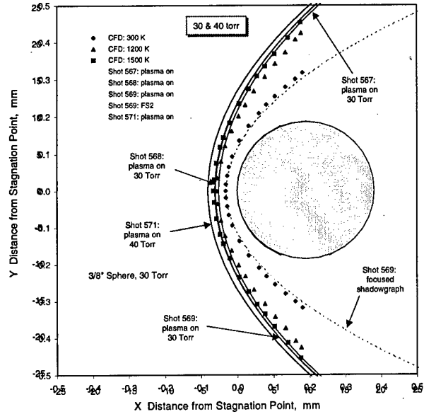
Figure 17. Comparison of curve fit data to CFD calculations (9.5-mm sphere).
