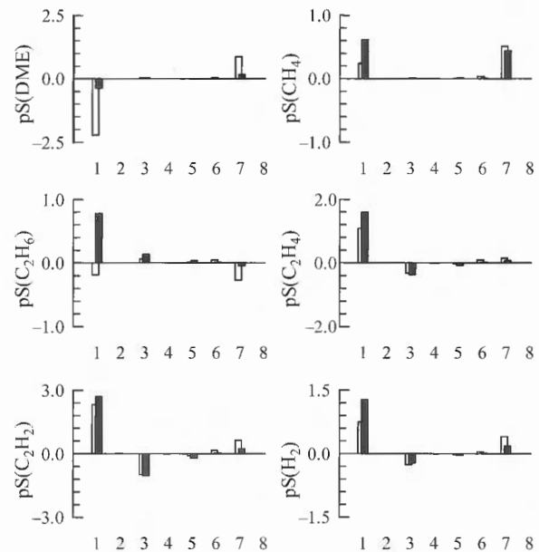
Fig. 1b. Sensitivity spectra (pS) [30] for DME, C 2 H 6 , C 2 H 4 , C 2 H 2 , CH 4 , and H 2 concentrations at 1300 K at 1000 \mu s using mixture A7. The solid bars show the result of multiplying the indicated rate constants by 0.2, while the open bars show the result of multiplying the indicated rate constants by 5. The horizontal axis shows the reaction numbers.
