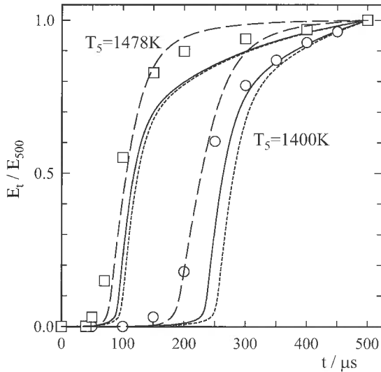
Fig. 8a. Comparison of the CO 2 profiles measured at 4.24 μm with those calculated using mixture A9. ○, observed at 1400 K, 1.94 atm and total density, 1.69 × 10 -5 mol/cm 3 ; □, observed at 1478 K, 2.12 atm and total density, 1.75 × 10 -5 mol/cm 3 ; —, calculated using DMEH-mec; ·····, calculated using DMEH-mec changing the k 3 value to k 3 = 4.8 × 10 7 T 1.9 exp (- 3.7 kcal/RT) cm 3 mol -1 s -1 ; ---, calculated using Fischer et al. mechanism [4].
