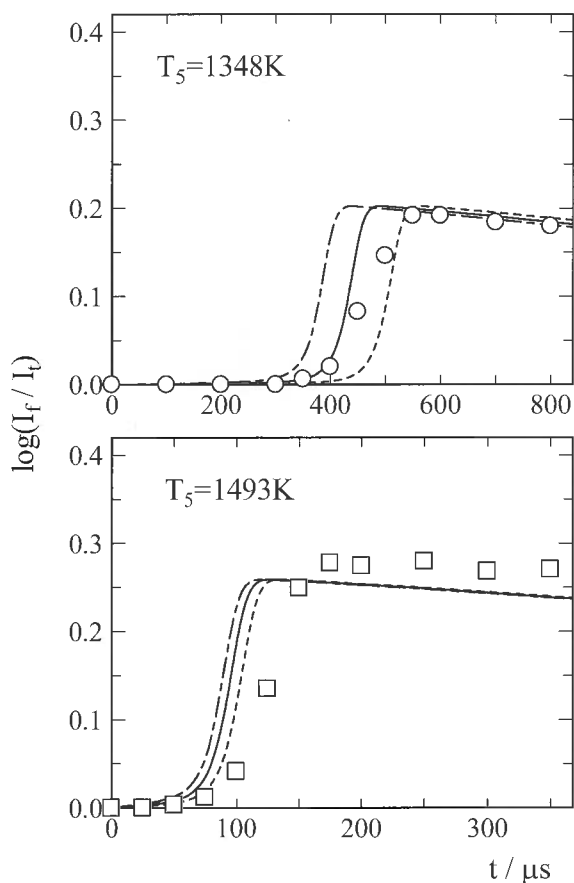
Fig. 12a. Comparison of the time-profiles measured at 306.7 nm with those calculated using mixture A13. \circ , observed at 1348 K, 1.60 atm and total density, 1.45 \times 10^{-5} \text{ mol/cm}^3 ; \square , observed at 1493 K, 1.89 atm and total density, 1.54 \times 10^{-5} \text{ mol/cm}^3 ; —, calculated using DMEH-mec; ---, calculated using DMEH-mec changing the k_3 value to reported maximum value k_3 = 4.8 \times 10^7 T^{1.9} \exp(-3.7 \text{ kcal/RT}) \text{ cm}^3 \text{ mol}^{-1} \text{ s}^{-1} [20]; -·-·-, calculated using DMEH-mec changing the k_5 value to k_5 = 9.35 \times 10^5 T^{2.29} \exp(0.78 \text{ kcal/RT}) \text{ cm}^3 \text{ mol}^{-1} \text{ s}^{-1} [4].
