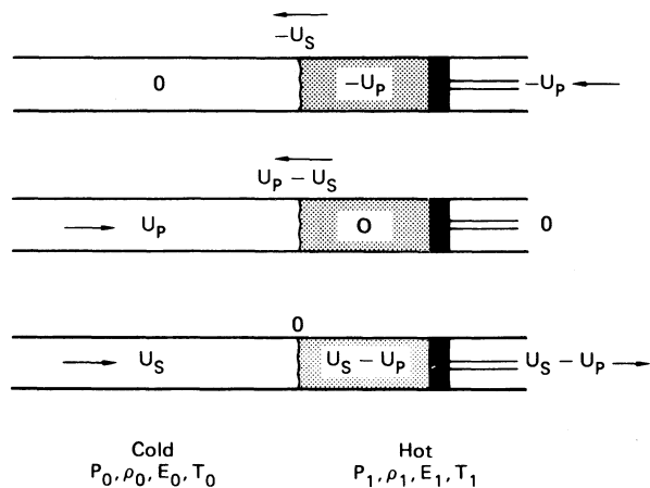
FIG. 2. Steady fluid shock waves viewed in three different coordinate frames. In the topmost frame the piston at the right moves to the left, compressing and heating the cold fluid. In the middle frame the piston is fixed and cold fluid moves to the right. The frame at the bottom of the figure fixed on the shock wave leads to the simple conservation equations solved in the text.
