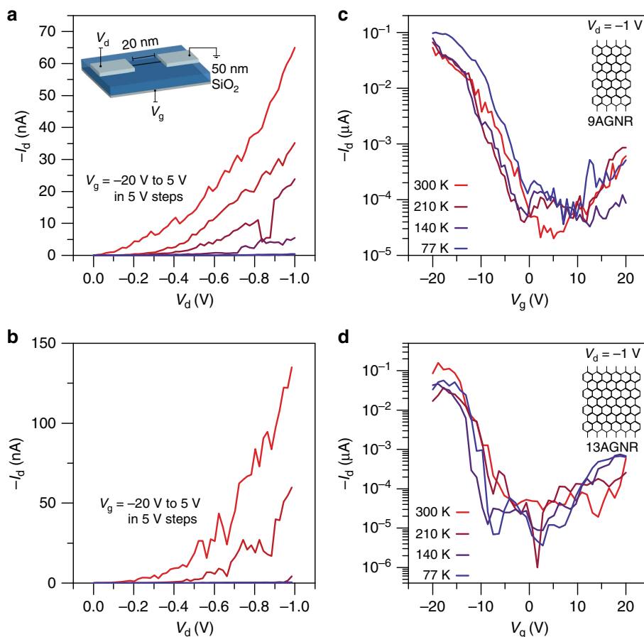
Fig. 3 Transport characteristics of 9AGNRs and 13AGNRs gated with 50 nm \text{SiO}_2 gate oxide. The presence of a SB is confirmed by non-linear current behavior at low drain bias and lack of current saturation at high drain bias for both a 9AGNRs and b 13AGNRs. The weak temperature dependence in the I_d - V_g behavior in c 9AGNRs and d 13AGNRs indicates that tunneling through the Pd-GNR SBs is the limiting transport mechanism of the device
