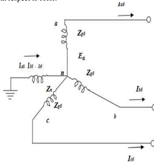
Fig:3 Negative Sequence Network
