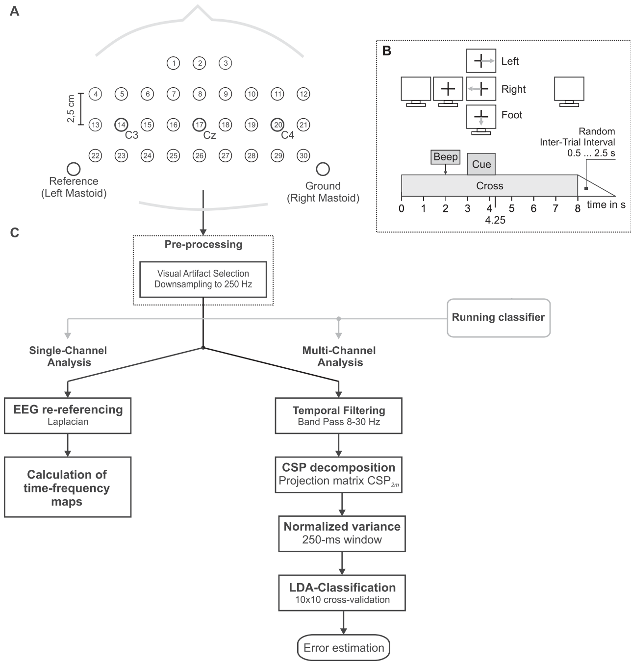
FIG. 1. Electrode positions (A), timing and cue-based experimental paradigm (B), and flow diagram of the data analysis (C). CSP, common-spatial pattern; LDA, linear discriminant analysis.
