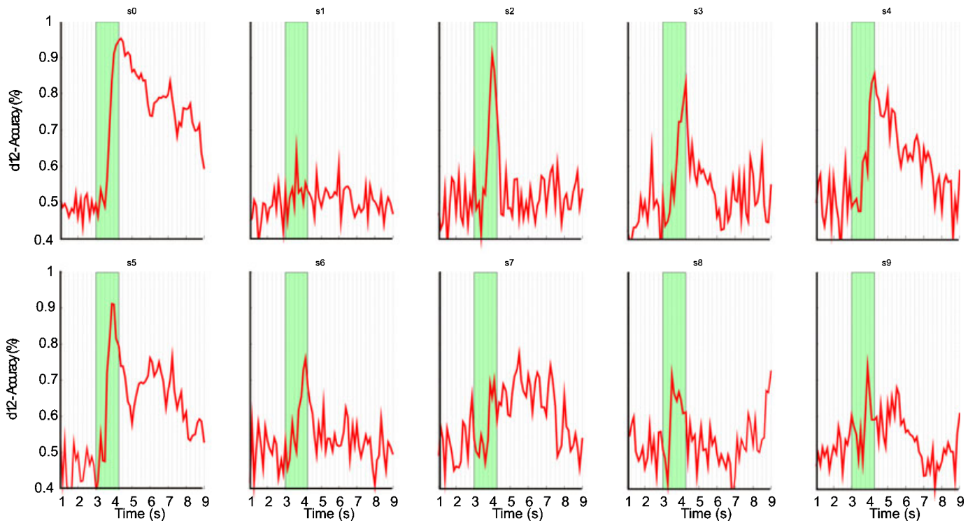
FIG. 2. Discrimination time courses documenting the separability between two brain states (right vs. left hand motor imagery) obtained with a 250-ms window. The time of visual cue presentation is indicated by a green bar. Classification accuracy from 40% to 100% is shown on the y-axis, and time from 1 s to 9 s appears on the x-axis. The data were collected from 10 naïve subjects without any motor imagery experience.
