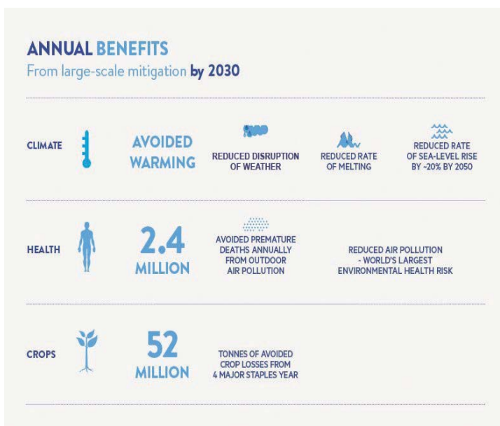
Figure 2 - Estimated annual benefits by 2030 from SLCP mitigation. Source CCAC http://www.ccacoalition.org/
