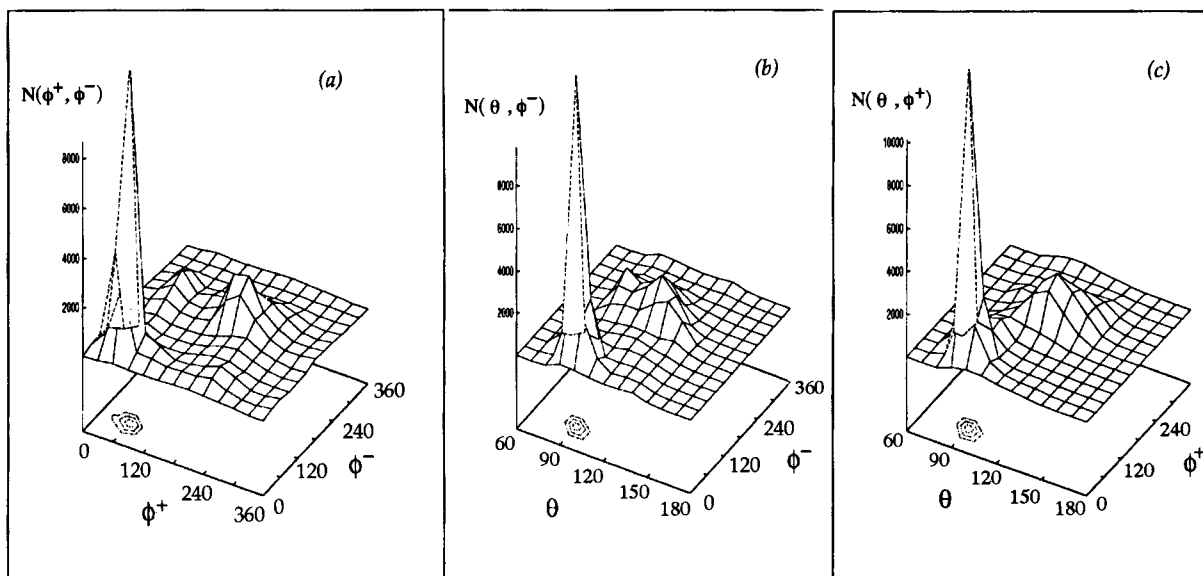
Fig. 4. Number distributions of pairs interdependent angles ( \phi^+ , \phi^- ), ( \theta , \phi^- ) and ( \theta , \phi^+ ), collected for all residue types in a set of previously reported 3 150 PDB structures. The doublet distribution N(\phi^-, \phi^+) is determined by considering regions of size ( \Delta\phi^-, \Delta\phi^+ ) = (30°, 30°). The region about ( \phi^-, \phi^+ ) \approx (60°, 60°) is
