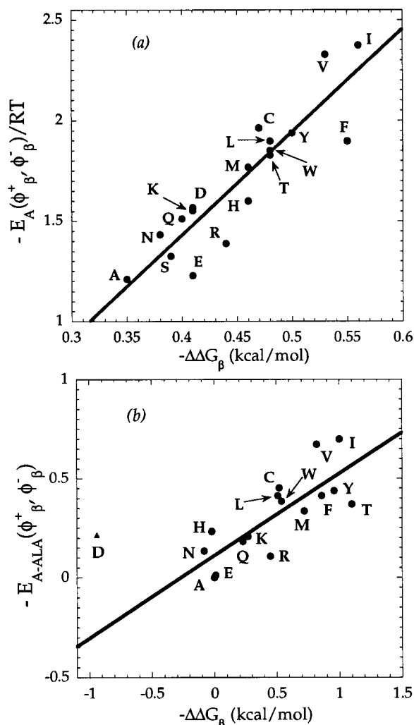
Fig. 9 a: Comparison of the \beta -sheet propensities of amino acids obtained by experiments and in the present analysis. The abscissa and ordinate, respectively, to the experimental results of Kim and Berg 38 and to the torsional energies E_A(\phi^+, \phi^-)/RT listed in the last column of Table II. The correlation coefficient between the two data sets is R = 0.90 . b: \beta -sheet propensities of amino acids obtained by experiments and in the present analysis. The abscissa represents the thermal stability measurements of Minor and Kim. 41 The ordinate follows from Table II, using E_{A-ALA}(\phi^+, \phi^-) \equiv E_A(\phi^+, \phi^-) - E_{ALA}(\phi^+, \phi^-) at 300K. The value R = 0.79 is obtained, excluding the data for Asp.
