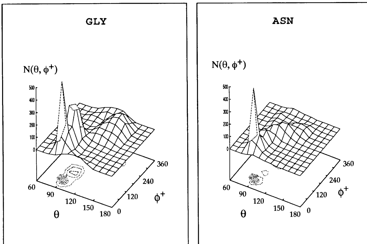
Fig. 6. N_A(\theta, \phi^+) for A = \text{Gly} and \text{Asn} reflecting the specificity of the coupling between the virtual bond angle \theta and the pseudodihedral \phi^+ .
