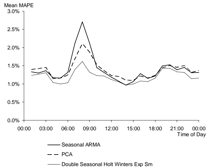
Fig. 5. For three hour-ahead prediction, Mean MAPE for the 10 load series plotted against time of day.
