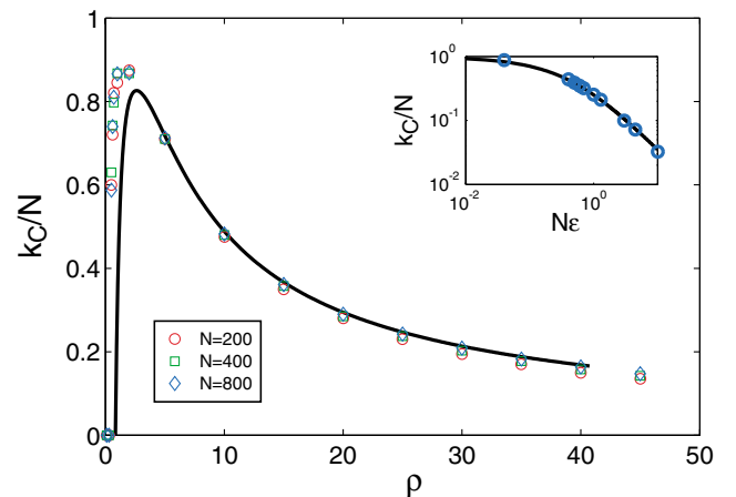
FIG. 3 (color). Capacity per neuron k_C as a function of \rho = N(1 - \alpha) , at \bar{\epsilon} = 0.04 , showing nonmonotonic dependence. Points from simulations on differently sized systems fall on essentially the same curve, confirming that in this regime capacity is extensive. The inset shows the dependence of k_C/N on scaled noise \bar{\epsilon} for \rho^{\text{opt}} both in the AA and from simulation.
