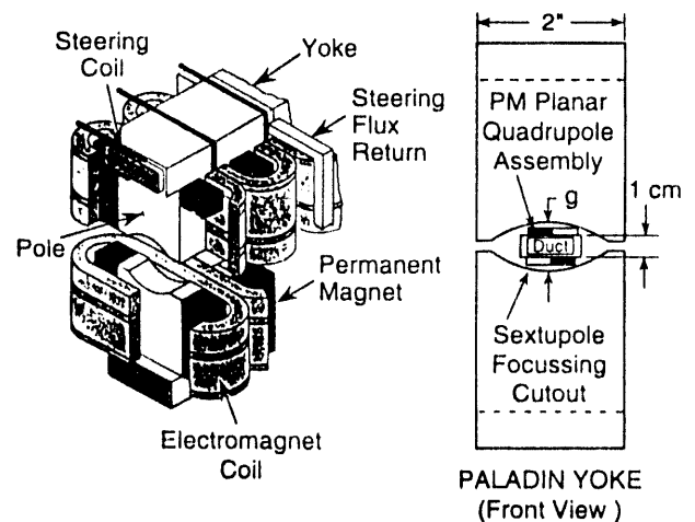
Fig. 6: Planar permanent magnet quadrupole in PALADIN.
