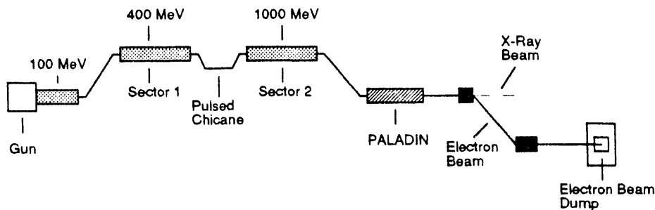
Fig. 5: Schematic overview of the demonstration experiment..
