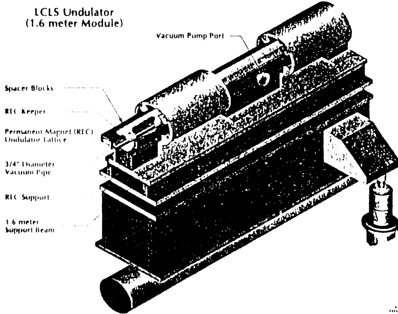
Fig. 3: LCLS undulator.
