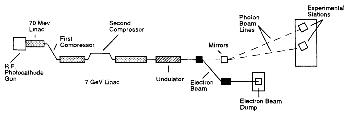
Fig. 1: LCLS overview.
