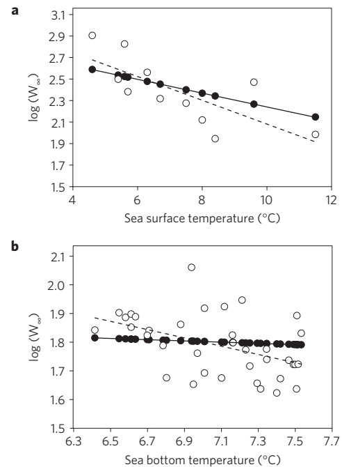
Figure 4 | Comparison of relationship between maximum body size ( W_{\infty} ) and habitat temperature predicted from the growth model presented in this study (filled dots, solid line) and observations (open dots, broken line). a , Maximum body weight for Atlantic cod ( Gadus morhua ) in the North Atlantic based on growth parameters estimated from body size-at-age data from populations in different locations in ref. 28, and b , maximum body weight for North Sea haddock ( Melanogrammus aeglefinus ) (based on growth parameters in ref. 11). The slopes of the best fit lines from linear regression for both datasets are significant ( p < 0.05 ). In both cases, the predicted changes in maximum body weight (log) over temperature are more conservative than the observed changes.
