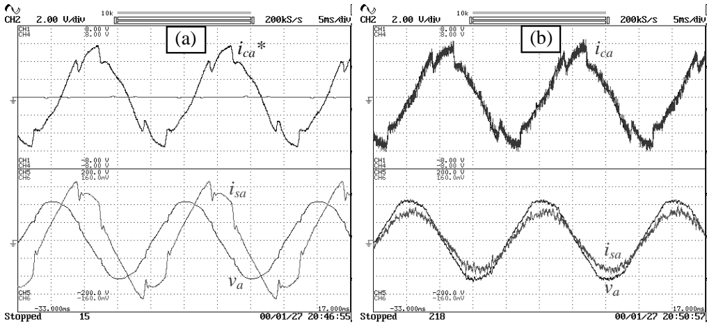
Fig. 10 - Power system with non-linear load: (a) Active filter inverter off; (b) Active filter inverter on.
