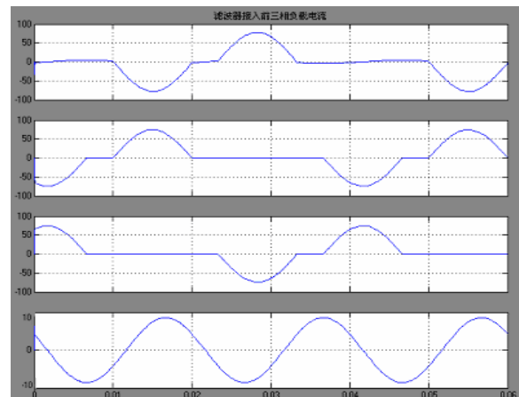
Fig.7. Currents before compensating
