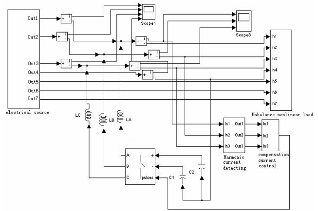
Fig.4. SAPF system simulation construction
