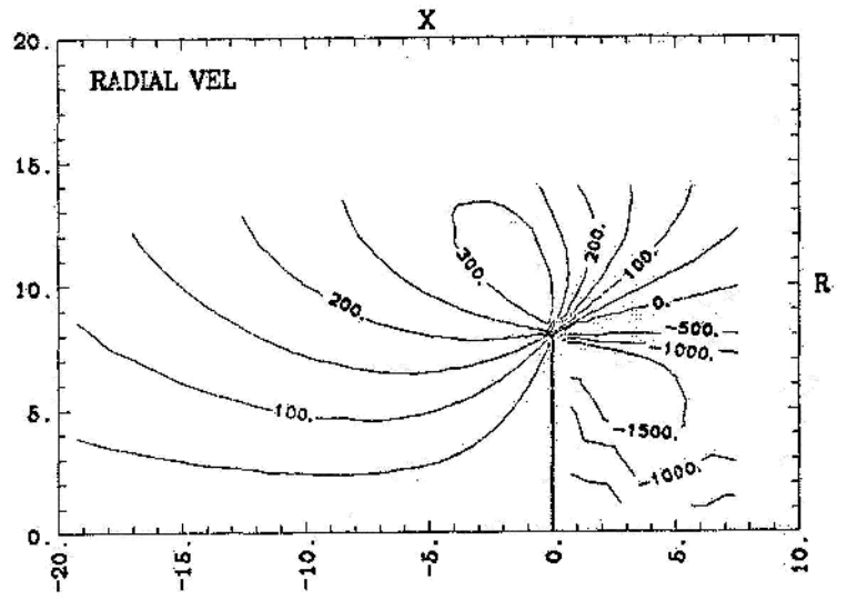
Fig. 1. Contours of flowfield properties, modeled shuttle fin.
