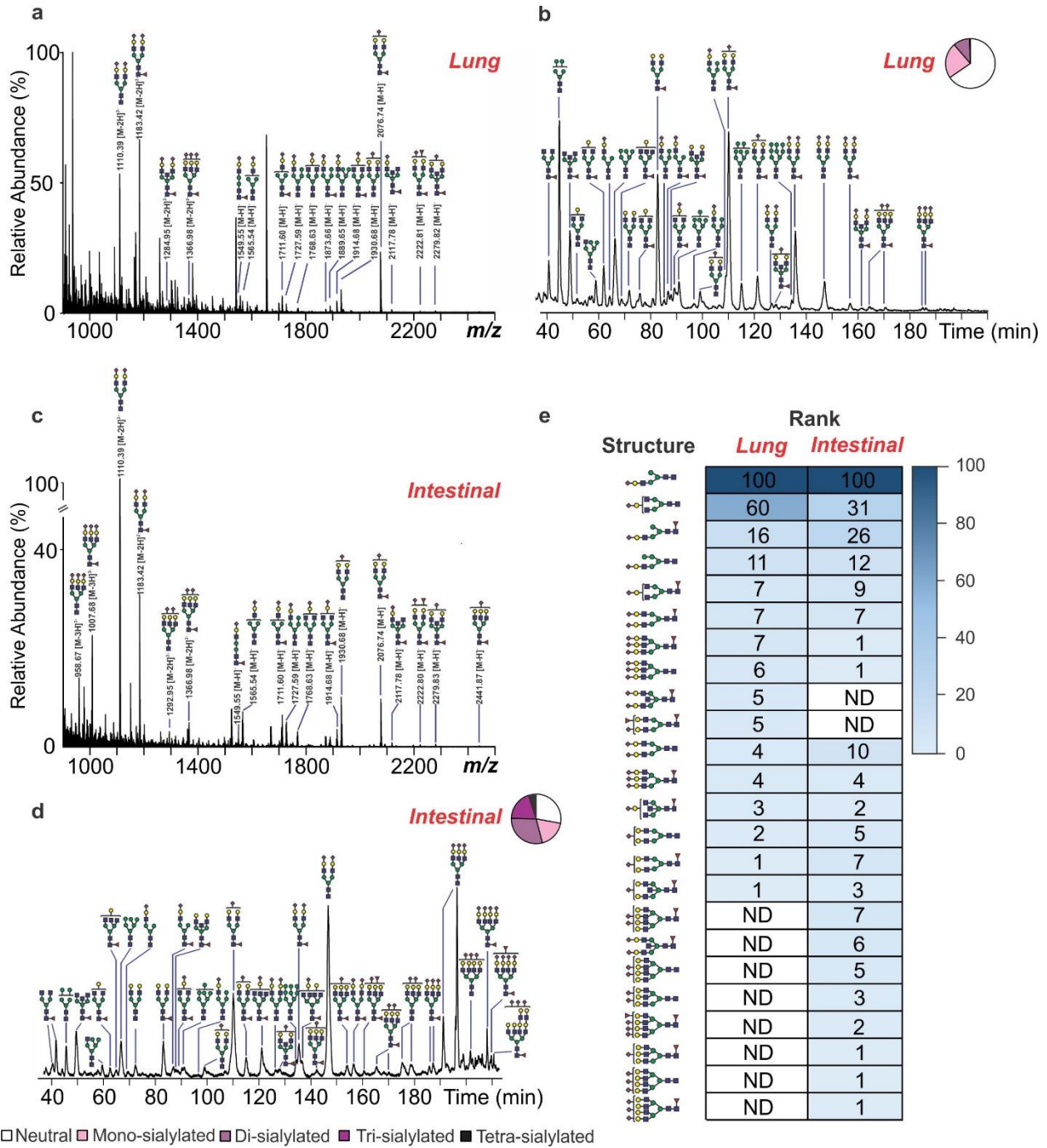
Figure 2. Screening of natural N -glycan libraries against RBD. a,c , CaR-ESI-MS screening results obtained for aqueous ammonium acetate solutions (100 mM, pH 6.9, 37 °C) of RBD (10 \mu M), P dimer of the Saga strain ( P_{ref} , 4 \mu M) and the N -glycan library from lung (200 \mu g/mL) ( a ) and intestinal (125 \mu g/mL) ( c ) tissues. Ions with m/z of 3000 – 4000 were subjected to HCD using a collision energy of 50 V. b,d , Chromatogram of 2-AB-labeled N -glycans released from lung ( b ) and intestinal ( d ) tissues acquired using HILIC-UHPLC with fluorescence detection. The relative abundances of the Neu5Ac content of the N -glycans are indicated graphically. e , Heat maps of relative affinities of ligands identified by CaR-ESI-MS screening at 37 °C; ND \equiv not detected.
