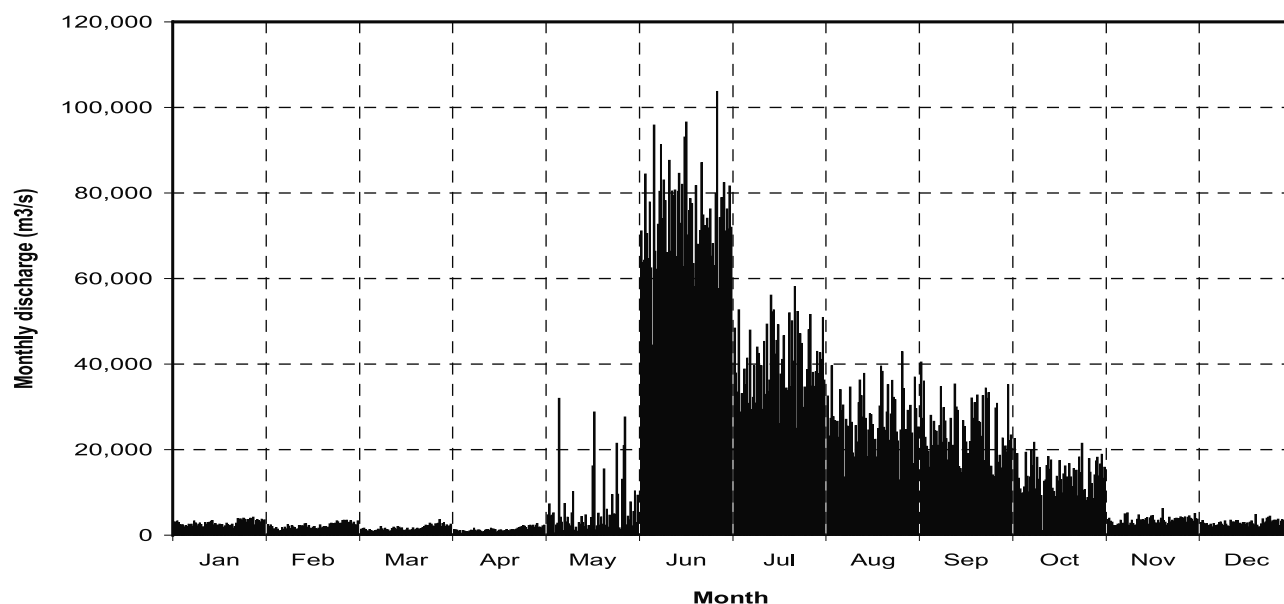
Figure 2. Monthly discharge during 1935–1999 at Kusun station of the Lena River. Note each bar in the graph representing an individual monthly value for each year during 1935–1999.
