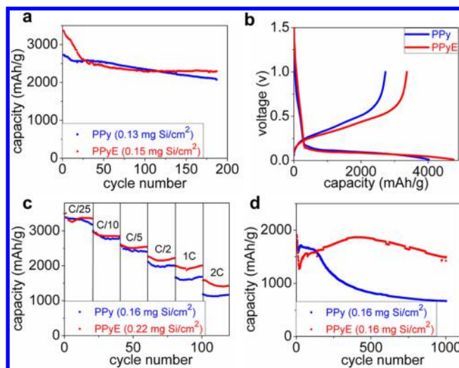
Figure 4. (a) Charge (delithiation) capacities of PPy- and PPyE-based Si electrodes at C/10. (b) First-cycle voltage curves. (c) Rate performance. (d) Charge (delithiation) capacities of PPy- and PPyE-based Si electrodes at 2C rate. Mass loadings of Si for each cell are labeled in the plot.
