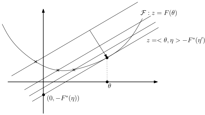
Fig. 3. Legendre transformation of a strictly convex function F : The z -intercept (0, -F^*(\eta)) of the tangent hyperplane H_\theta : z = \langle \eta, \theta \rangle - F^*(\eta) of the potential function defines the value of the Legendre transform F^* for the dual coordinate \eta . Any hyperplane passing through another point of the potential function and parallel to H_\theta necessarily intersects the z -axis above -F^*(\eta) .
