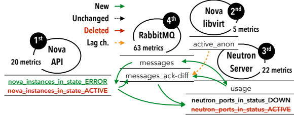
Figure 8. Final edge differences for RCA evaluation between top 5 components of Table 5 with similarity threshold of 0.50.
