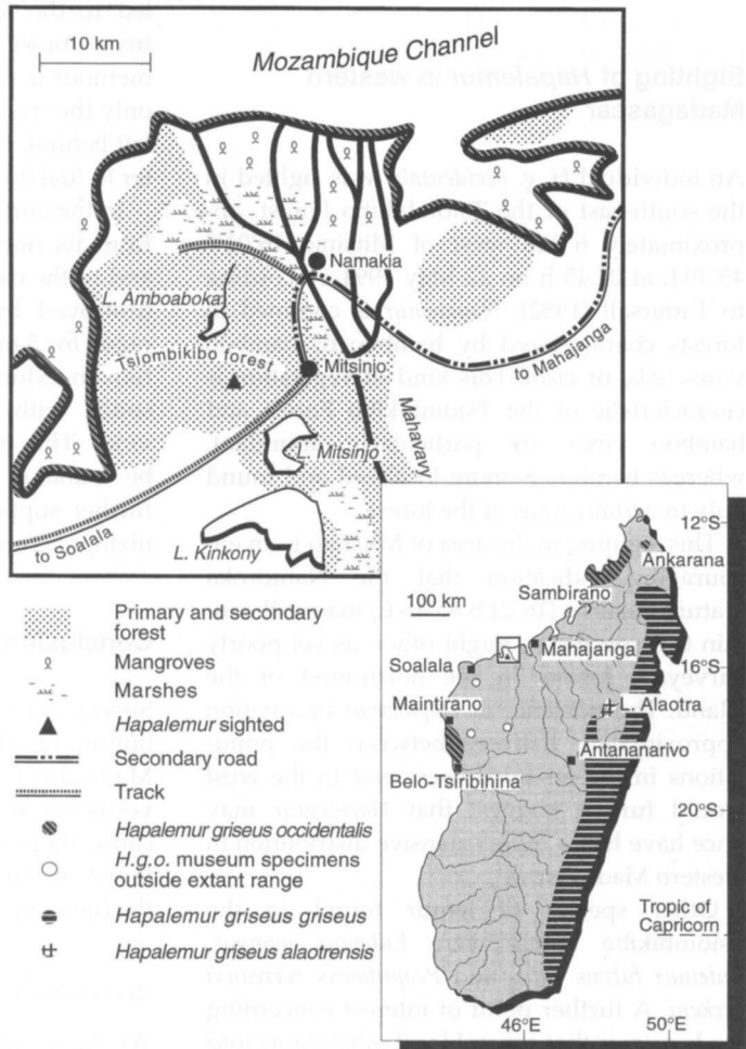
Figure 1. Distribution of Hapalemur griseus and sighting of Hapalemur griseus occidentalis ( Hgo ). Adapted from: Tattersall (1982); Carte de Madagasikara 1:500 000 (Anon., 1986); Nicoll and Langrand (1989); Mittermeier et al. (1992).
