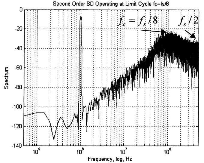
Fig. 6. SD operating on limit cycle with \omega_c = \omega_s/8 .
