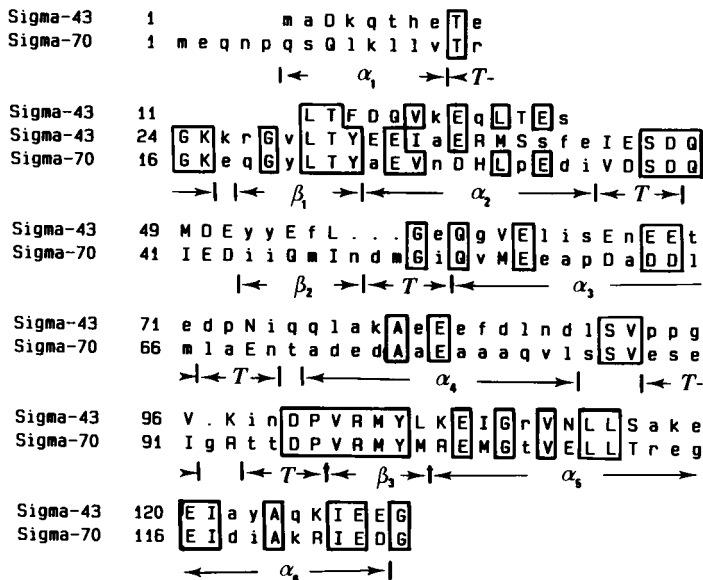
Figure 3. Alignment of Sigma-43 and Sigma-70 in Region 1.
