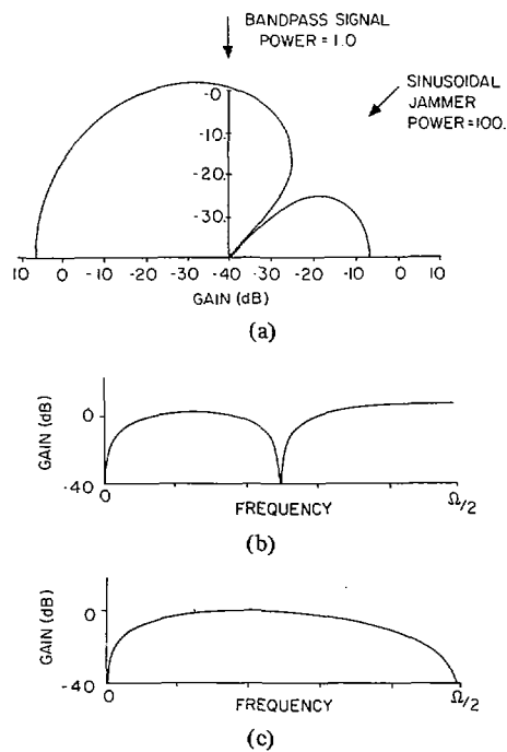
Fig. 7. Behavior of "converged" Howells-Applebaum sidelobe canceller. (a) Antenna pattern plotted at jammer frequency. (b) Frequency response in jammer direction. (c) Frequency response in signal direction.
