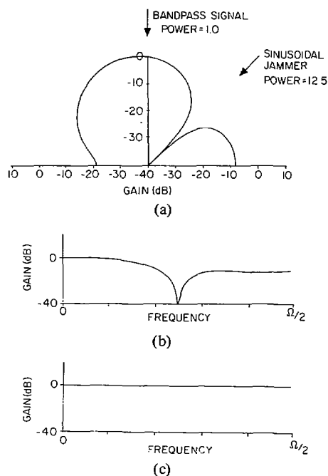
Fig. 10. Behavior of "converged" Frost beamformer. (a) Antenna pattern plotted at jammer frequency. (b) Frequency response in jammer direction. (c) Frequency response in signal direction.
