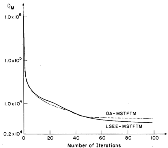
Fig. 4. D_M versus iteration number of LSEE-MSTFTM and OA-MSTFTM.
