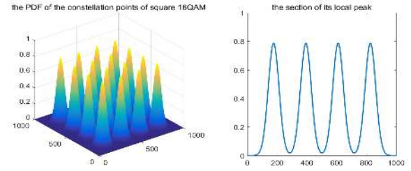
Fig. 1. The probability density function of the constellation point of square 16QAM and the section of its local peak
