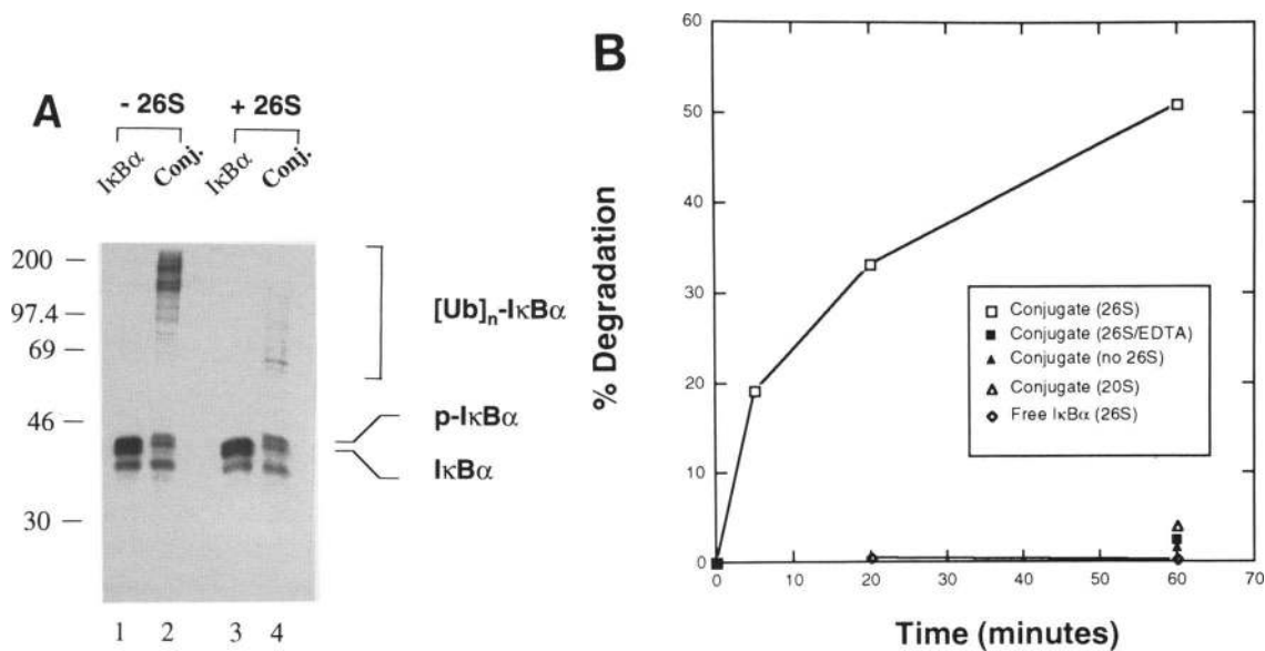
Figure 5. Degradation of ubiquitinated I \kappa B \alpha by the 26S proteasome. (A) In vitro-translated ^{35} S-labeled I \kappa B \alpha was incubated in HeLa extracts at 37°C for 2 hr under ubiquitination conditions (see Materials and methods), except that either Mg-ATP (lanes 2,4) or EDTA (lanes 1,3) was added to the reaction. The reaction mixtures were then immunoprecipitated by an antibody against RelA under conditions that allow coprecipitation of conjugated (lanes 2,4) or unconjugated (lanes 1,3) I \kappa B \alpha . The immunoprecipitates were then used directly for the degradation assay by the 26S proteasome. Lanes 1 and 2 are minus (-) 26S; lanes 3 and 4 are plus (+) 26S (23 nM). The degradation reactions were carried out at 37°C for 1 hr in the presence of Mg-ATP, and the reaction mixtures were separated by SDS-PAGE, followed by fluorography. (B) Ubiquitinated I \kappa B \alpha in the immunoprecipitates described in A (lane 2) was incubated with 26S proteasome (17 nM) at 37°C in the presence of Mg-ATP ( \square ). At indicated time points, an aliquot of the reaction was precipitated by 10% TCA. The TCA-soluble radioactivity was then determined by liquid scintillation counting. Similarly, degradation of unconjugated (free) I \kappa B \alpha was also determined ( \diamond ). In other reactions, 40 mM EDTA was added ( \blacksquare ), 26S proteasome was omitted ( \blacktriangle ), and 20S proteasome (49 nM) was added ( \triangle ) instead of the 26S proteasome.
