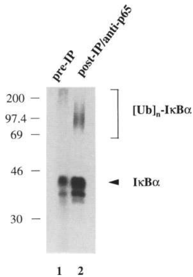
Figure 3. Association of ubiquitinated I \kappa B \alpha with NF \kappa B. Conditions for the synthesis of ubiquitinated I \kappa B \alpha were as described in Fig. 2A except that the reaction was carried out at 37°C for 2 hr. Ten percent of the reaction mixture was saved for SDS-PAGE analysis (lane 1), and I \kappa B \alpha in the remaining mixture was coimmunoprecipitated with RelA using antisera against RelA/p65 (see Materials and methods). The precipitates were boiled in SDS sample buffer, followed by SDS-PAGE and fluorography (lane 2). An amount equivalent to ~50% of the initial reaction volume was loaded in lane 2, which is fivefold greater than that loaded in lane 1. The bulk of the high molecular mass conjugates in lane 2 is approximately 100 kD, as opposed to 200 kD seen in lane 1, and this may be attributable to “trimming” by isopeptidases during the immunoprecipitation.
