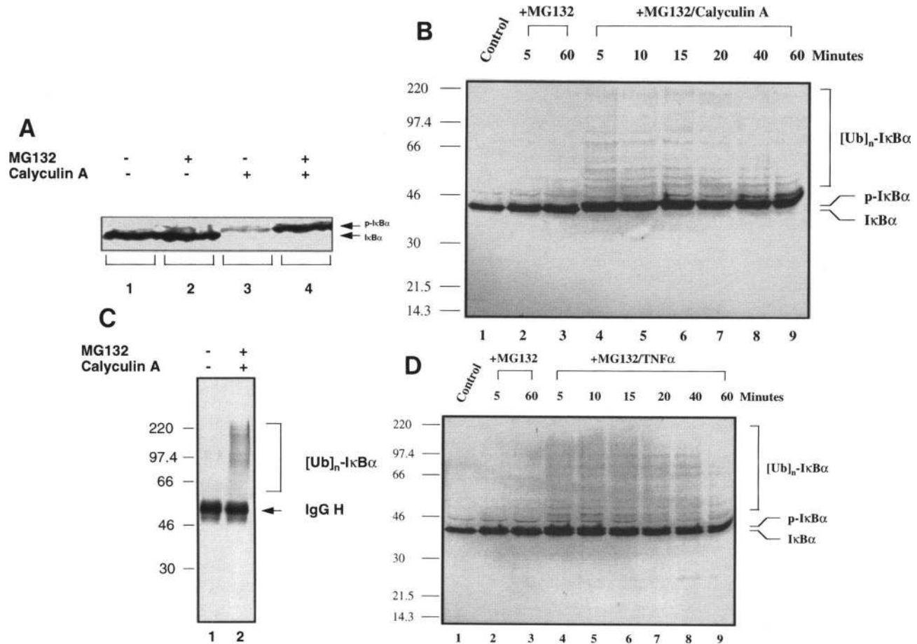
Figure 1. Induced phosphorylation and ubiquitination of I \kappa B \alpha in calyculin A or TNF \alpha -treated cells. (A) Stabilization of the phosphorylated form of I \kappa B \alpha by MG132. Jurkat T cells were pretreated with 40 \mu M of MG132 (lanes 2,4) or DMSO (a diluent for MG132, lanes 1,3) for 30 min before incubation with 0.3 \mu M of calyculin A (lanes 3,4) or DMSO (lanes 1,2) for an additional 30 min. Cytoplasmic extracts were prepared, fractionated by SDS-PAGE, and analyzed by Western blot using a rabbit polyclonal antibody against the carboxyl terminus of I \kappa B \alpha (amino acids 297–317, c-21). The phosphorylated form of I \kappa B \alpha is designated p-I \kappa B \alpha . (B) Induced ubiquitination of I \kappa B \alpha by calyculin A. Jurkat T cells were pretreated with MG132 (40 \mu M, lanes 2–9) or DMSO (lane 1) for 30 min before addition of calyculin A (0.3 \mu M, lanes 4–9) or DMSO (lanes 2,3). Cell extracts were prepared at 5 min (lanes 2,4), 10 min (lane 5), 15 min (lane 6), 20 min (lane 7), 40 min (lane 8), and 60 min (lanes 3,9) after adding calyculin A or DMSO. The extraction buffers contained RIPA/0.1% SDS plus 5 mM N -ethylmaleimide (NEM). The extracts were then subjected to Western blot analysis as described in A. (C) Jurkat T cells were treated as described in lanes 1 and 4 in A, except that cytoplasmic extracts were first immunoprecipitated with an antibody against the carboxyl terminus of I \kappa B \alpha (see Materials and methods). The immunoprecipitates were then eluted with 0.1 M Capso (pH 11.2), and the eluates were separated by SDS-PAGE, followed by Western blotting with a rabbit polyclonal antibody (anti-Ub) that specifically recognizes ubiquitin conjugates. The arrow marked IgG H indicates rabbit immunoglobulin heavy chain in the immunoprecipitates that cross-reacts with the secondary antibody (alkaline phosphatase conjugated anti-rabbit Fc). (D) Induced ubiquitination of I \kappa B \alpha by TNF \alpha . Experiments were carried out as described in B, except that calyculin A was replaced with TNF \alpha (10 ng/ml).
