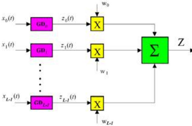
Figure 11. GR structure with L - 1 fingers.
