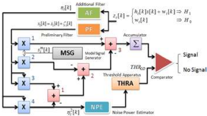
Figure 1. GR flowchart.
