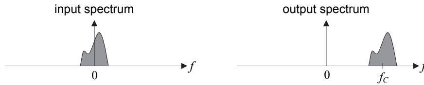
Fig. 14 An example of pure frequency translation using complex mixing.
