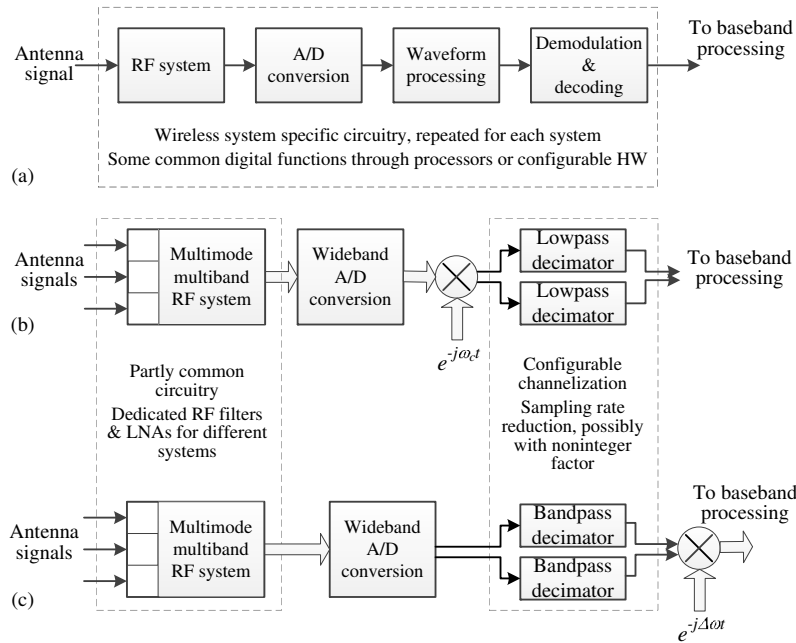
Fig. 23 Alternative multi-radio approaches. (a) Traditional receiver structure. (b) Configurable receiver based on digital I/Q mixing and baseband decimation filtering. (c) Configurable receiver based on bandpass decimation filtering and frequency offset compensation at low sample rate.
