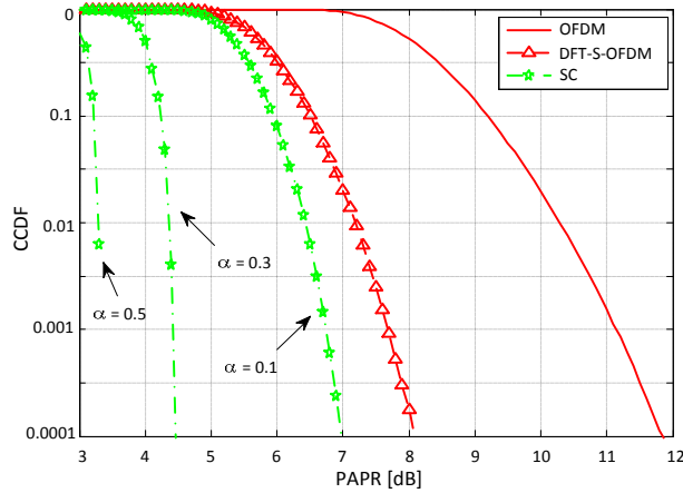
Fig. 7 Complementary cumulative distribution functions for the PAPR of OFDM, SC-FDMA, and single-carrier waveforms with different excess bandwidths. QPSK modulation, 160 subcarriers in OFDM and SC-FDMA. The roll-off parameter \alpha controls the signal bandwidth as (1 + \alpha)/T , where T is the symbol interval in traditional SC-transmission.
