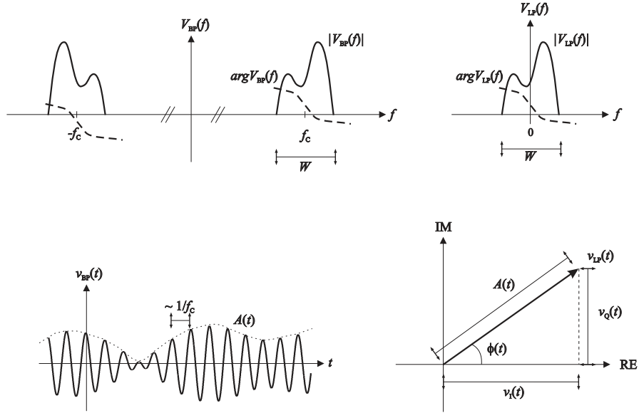
Fig. 11 Illustration of bandpass signal structure in time- and frequency domains. Left half shows a principal bandpass signal spectrum and the corresponding time-domain waveform. Right half, in turn, shows the corresponding lowpass equivalent signal spectrum and the corresponding time-domain complex signal as a time-varying phasor in complex plane.
