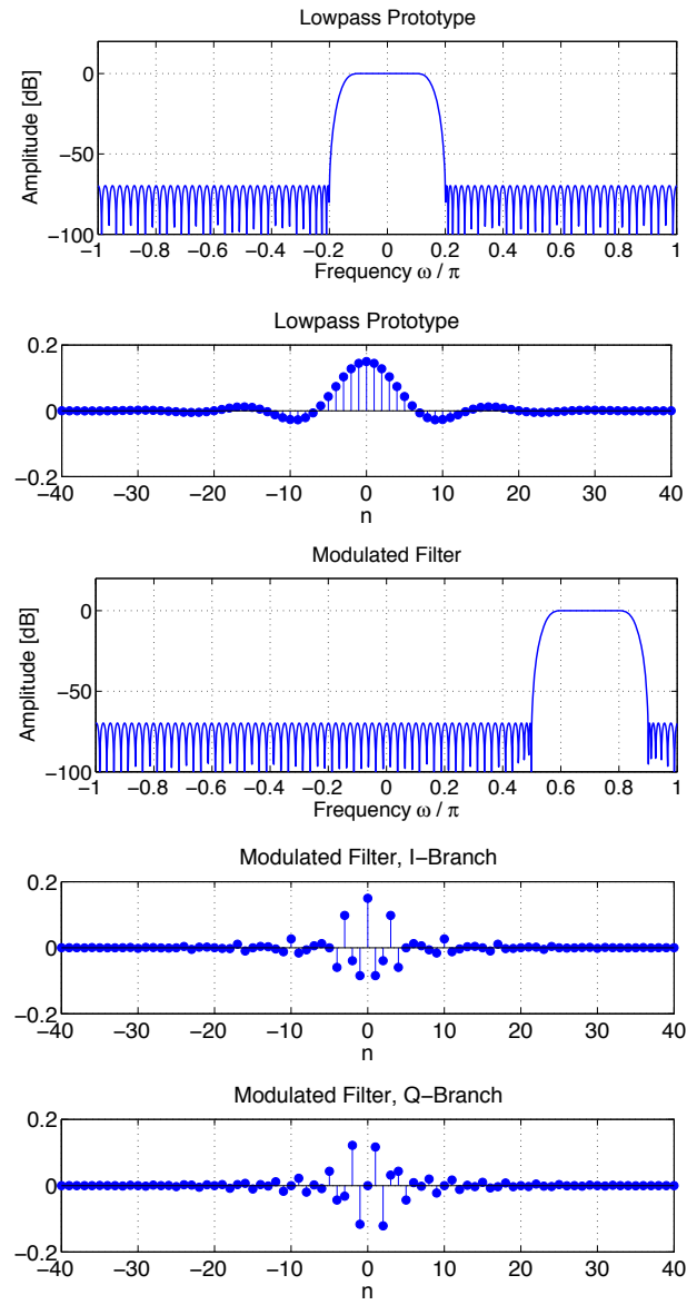
Fig. 18 An illustration of analytic bandpass filter generation through complex modulation of a lowpass prototype.
