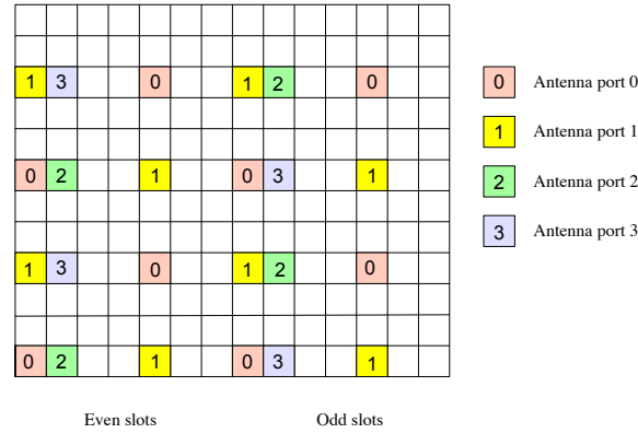
Fig. 3 Pilot symbol spacing in LTE standard for 4 \times 4 MIMO channel [91]. The figure shows 2 resource blocks, each consisting of seven QAM symbols (horizontal dimension) in 12 subcarriers (vertical dimension).
