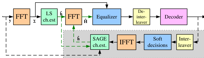
Fig. 4 Decision-directed channel estimation in MIMO receiver [91].
