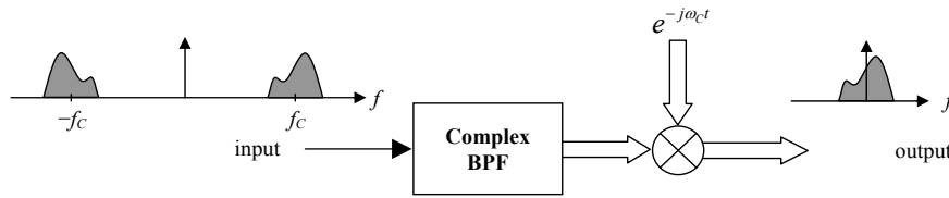
Fig. 19 An alternative structure for I/Q demodulation using complex bandpass filtering and complex downconversion.
