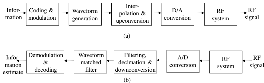
Fig. 1 Simplified wireless transceiver processing chain: (a) transmitter, (b) receiver.
