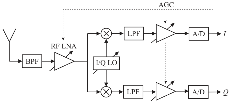
Fig. 22 Principal structure of direct-conversion radio receiver.
