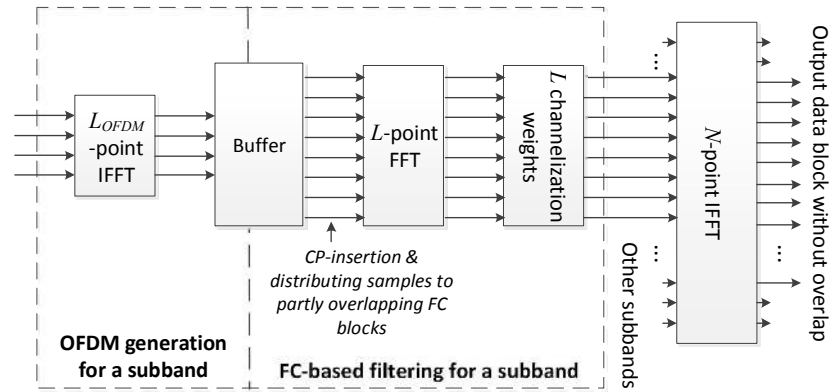
Fig. 10 Fast-convolution filtered OFDM transmitter structure.
