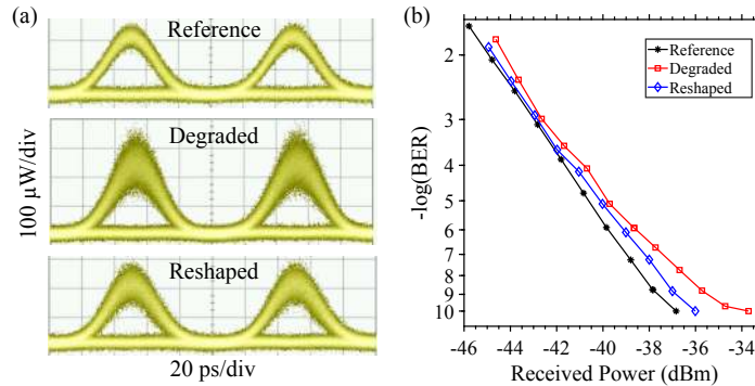
Fig. 7. Suppression of random intensity noise. (a) Eye diagrams of 10 Gbit/s RZ -OOK for the reference (top), degraded with random noise (middle) and reshaped (bottom) signals. (b) The BER measurements for signals shown in part (a).
