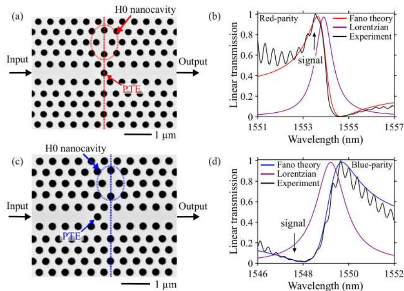
Fig. 3. Photonic crystal (PhC) Fano structures and resonance lineshapes. (a) Scanning electron microscope (SEM) image of the fabricated PhC with the PTE placed at the midplane passing through the cavity center. (b) Measured (black line) and simulated (red) transmission spectrum of the device in part (a) showing a red-parity Fano resonance. It is compared to the transmission of a Lorentzian (purple) resonance having the same Q-factor and resonance wavelength as the red-parity Fano resonance. (c) SEM of the device with the PTE placed one lattice constant to the left from the mid-plane. (d) Measured (black) and simulated (blue) transmission spectrum of the device in part (c) exhibiting a blue parity Fano resonance. It is compared with Lorentzian (purple) transmission having the same Q-factor and resonance wavelength as the blue-parity Fano resonance.
