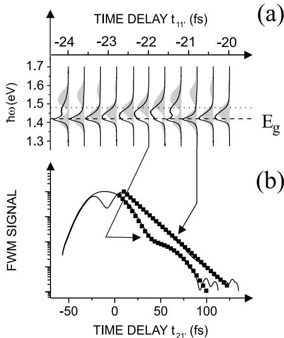
FIG. 2. Examples of experimental results presented as Fig. 1 (theory). (a) t_{21'} = 0 fs, the symbols in (b) are the result of simple fits. Bulk GaAs at T = 300 K excited by 13 fs pulses, n_{\text{eh}} = 5.4 \times 10^{17} \text{ cm}^{-3} . The oscillation period under these conditions is 68 fs.
