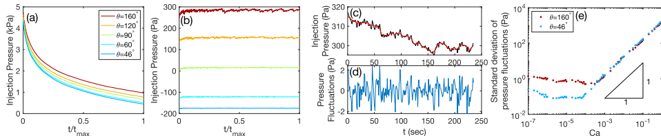
FIGURE 3. (a)-(b) Temporal evolution of the injection pressure at Ca = 10^{-3} and Ca = 10^{-7} respectively. At high Ca , the injection pressure decreases as the viscous fingers approach the outer boundary of the flow cell. At low Ca , the injection pressure is dominated by Laplace pressure fluctuations at the interface. We use wavelet decomposition (Cai 2002; Sygouni et al. 2006, 2007) to split the pressure signal ( Ca = 10^{-5} and \theta = 160^\circ here) into its (c) global trend and (d) cyclic component. (e) The standard deviation of the pressure fluctuations point at two different regimes. At low Ca , pressure fluctuations are dominated by stick-slip changes in Laplace pressure. At high Ca , pressure fluctuations are dominated by changes in the effective hydraulic conductance of dominant flow channels.
