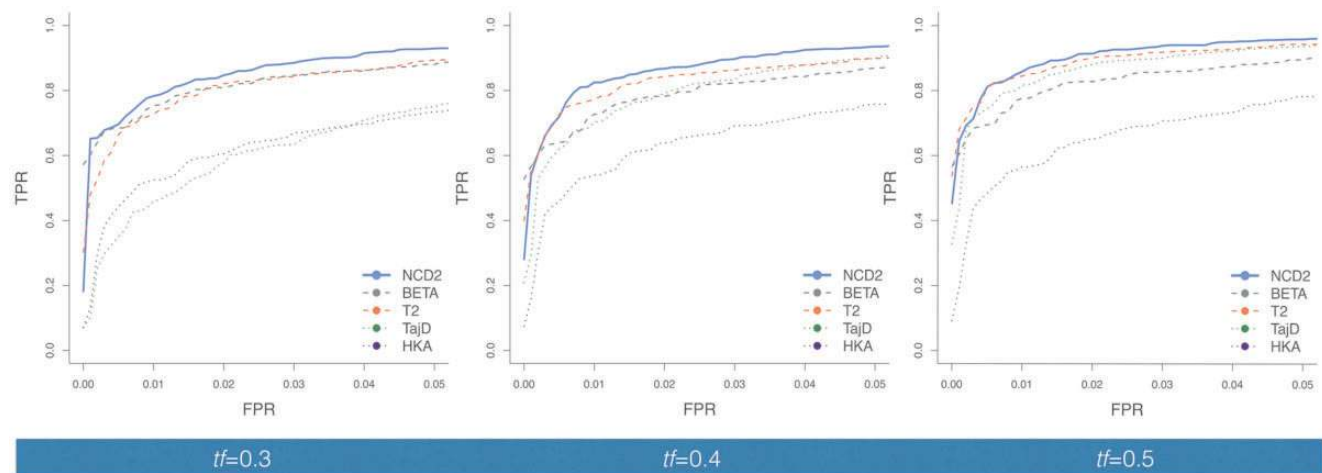
Fig. 2. —Power to detect balancing selection for NCD2(0.5) and other tests. The ROC curves summarize the true positive rate (TPR) as a function of the false positive rate (FPR) to detect LTBS for simulations where the balanced polymorphism was modeled to achieve f_{eq} of (A) 0.3, (B) 0.4, and (C) 0.5. Plotted values are for the African demography, Tbs = 5 Ma. L = 3 kb, except for T_1 and T_2 where L = 100 ISs (see Methods). BETA refers to the \beta statistic (Siewert and Voight 2017). For NCD2 calculations, tf = f_{eq} . European demography yields similar results (supplementary fig. S10, Supplementary Material online). Power for NCD1 , NCD1 + HKA , and T_1 is provided in supplementary table S1, Supplementary Material online.
