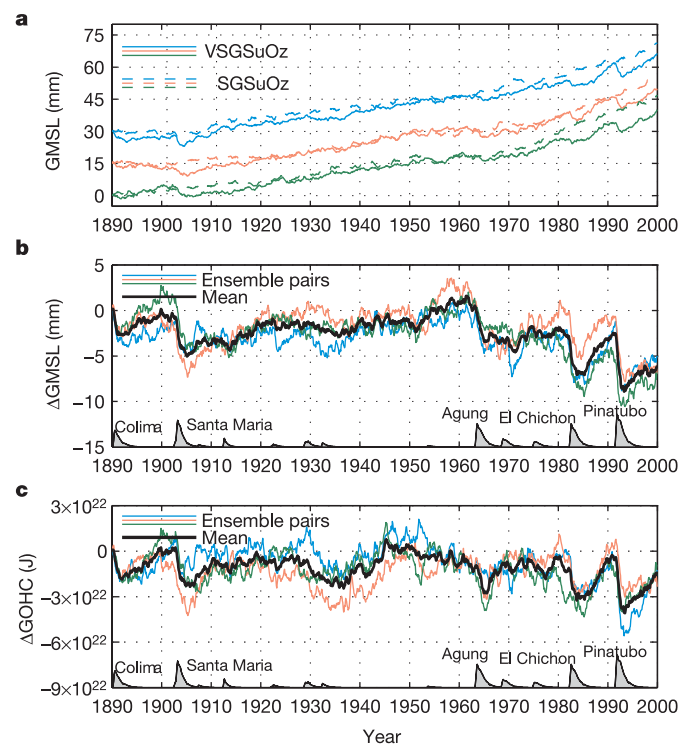
Figure 1 Changes in global mean sea level (GMSL) and global ocean heat content (GOHC) in the PCM simulations. a , Three pairs of simulations of full depth GMSL with time-varying volcanic, solar, greenhouse gases, sulphates and ozone ('VSGSuOz') forcing and the corresponding simulations without the volcanic forcing ('SGSuOz') are shown respectively by the solid and dashed lines. The differences between the pairs for GMSL ( \Delta GMSL; b ) and GOHC (upper 300 m only) ( \Delta GOHC; c ) are the coloured lines and the ensemble average is the bold black line. The global average optical depth (stratospheric optical depth at 0.5 \mu\text{m} ; ref. 12) is also shown (thin black line at bottom; arbitrary scale).
