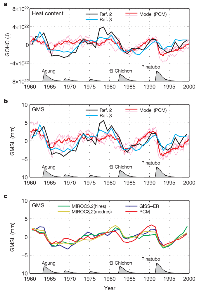
Figure 2 | Observed and modelled GOHC and GMSL for the period 1960–2000. The response to volcanic forcing, as indicated by the differences between the pairs of PCM simulations for GOHC ( a ) and the GMSL ( b ) is shown for the ensemble mean (bold line) and the three ensemble members (light lines). The observational estimates 2,3 of GOHC and GMSL are shown by the black and blue bold lines. For a and b , all results are for the upper 300 m only and have been detrended over the period 1960–2000. c , The ensemble mean (full depth) GMSL for the GISS-ER, MIROC3.2(hires), MIROC3.2(medres) and the PCM models (after subtracting a quadratic) are shown.
