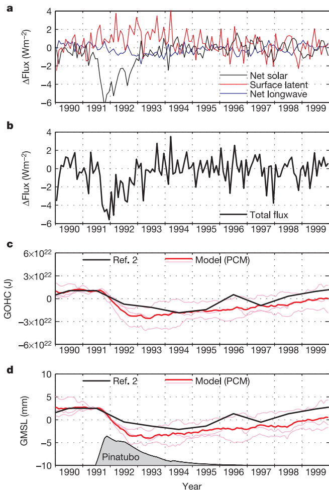
Figure 3 Ocean heat budget anomalies associated with the Mt Pinatubo eruption. a , The net solar (black), latent heat (red) and net long-wave (blue) heat fluxes. b , The total surface heat flux. Positive (negative) fluxes are a warming (cooling) of the ocean, and the fluxes are the averages of the differences between the three ensemble pairs. c , The modelled and observed 2 GOHC. d , The modelled and observed 2 GMSL. For c and d , the three ensemble pair differences between the models with and without volcanic forcing are shown as light lines, and the ensemble average bold, and are for the upper 300 m only.
