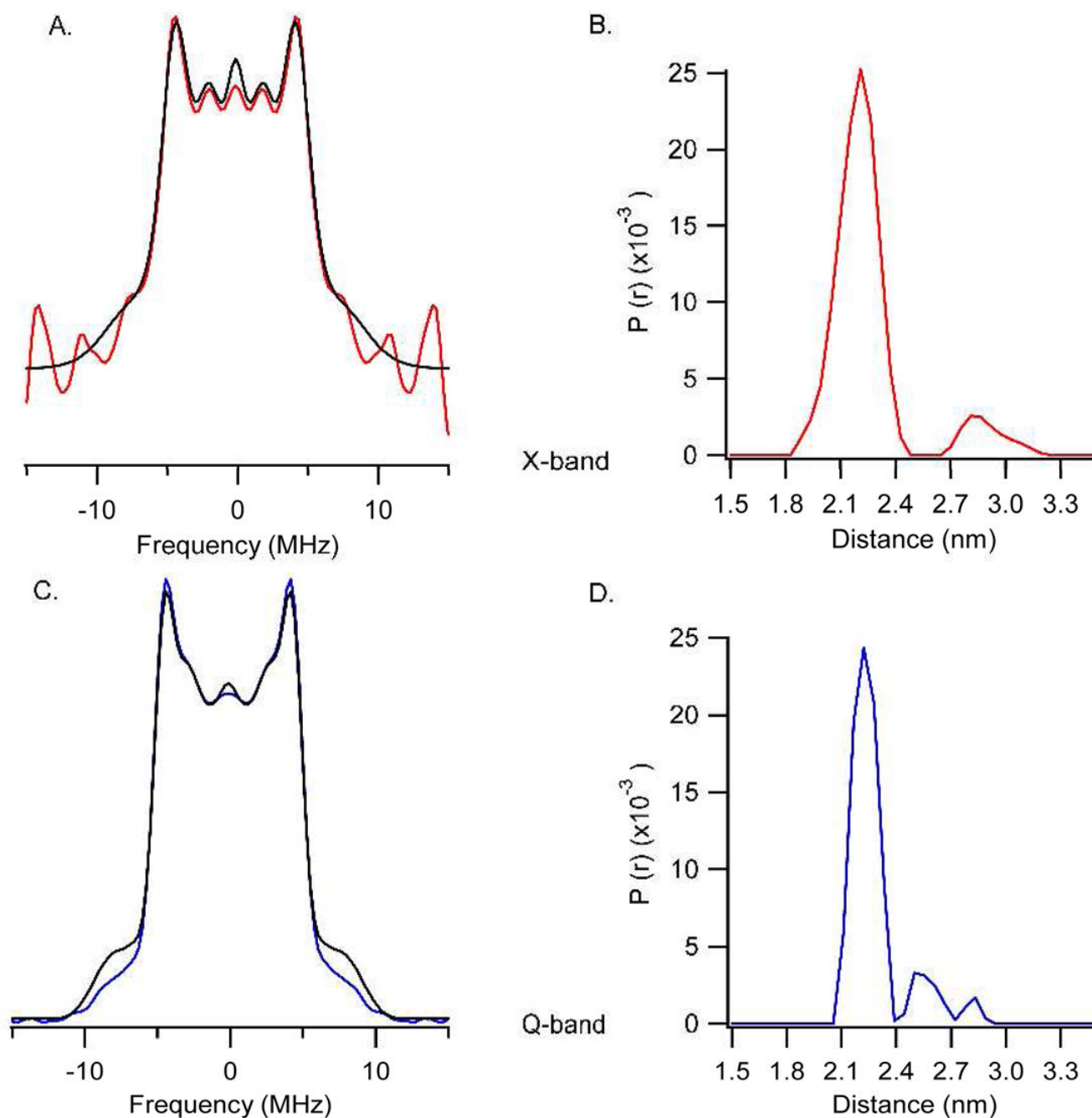
Figure 3. Frequency domain and distance distribution at X-band (Figs. 3A and 3B) and Q-band (Figs. 3C and 3D). X-band: zero time, 108 ns; phase, 30.4; background, 263 ns; regularization parameter 1; distance 2.27 nm; Q-band: zero time, 115 ns; Phase, 4.7; background, 348 ns; regularization parameter, 0.001; distance 2.32 nm. The simulations are shown in black.
