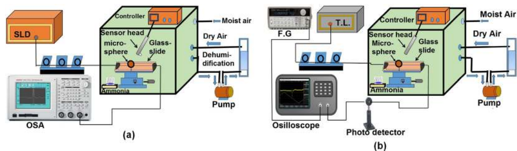
Figure 2. Experimental setup for ammonia sensing using (a) OSA interrogation system; (b) frequency detuning method.
