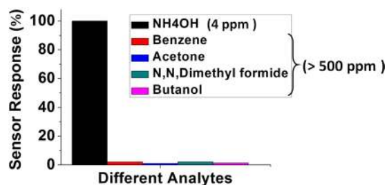
Figure 7. Sensor's response to various volatile organic compounds.
