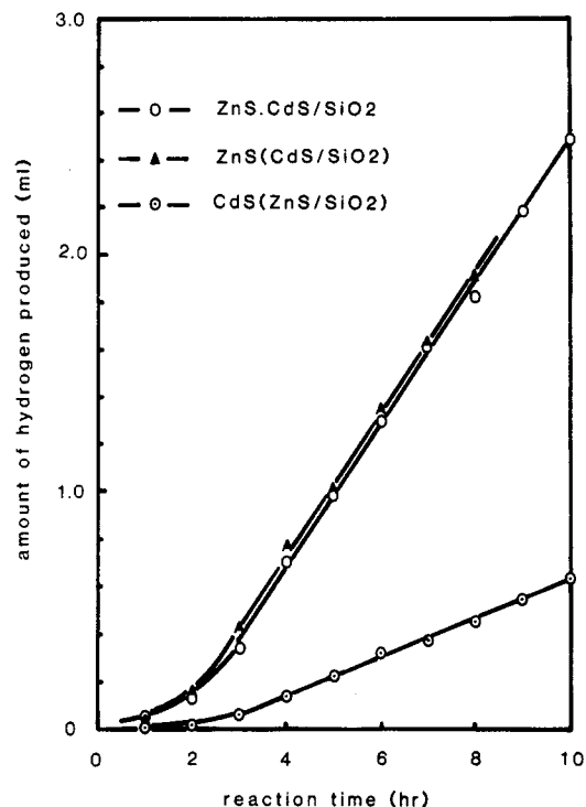
Figure 4. Amount of hydrogen produced by ZnS-CdS/SiO 2 , ZnS-(CdS/SiO 2 ), and CdS(ZnS/SiO 2 ) upon irradiation with UV-visible light. The amounts of ZnS and CdS in these three catalysts were the same.
