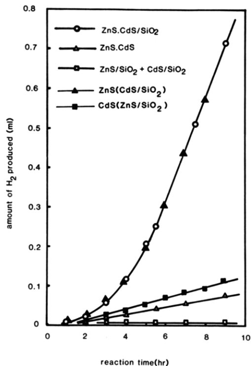
Figure 7. Amount of hydrogen produced by various catalysts with visible light.
