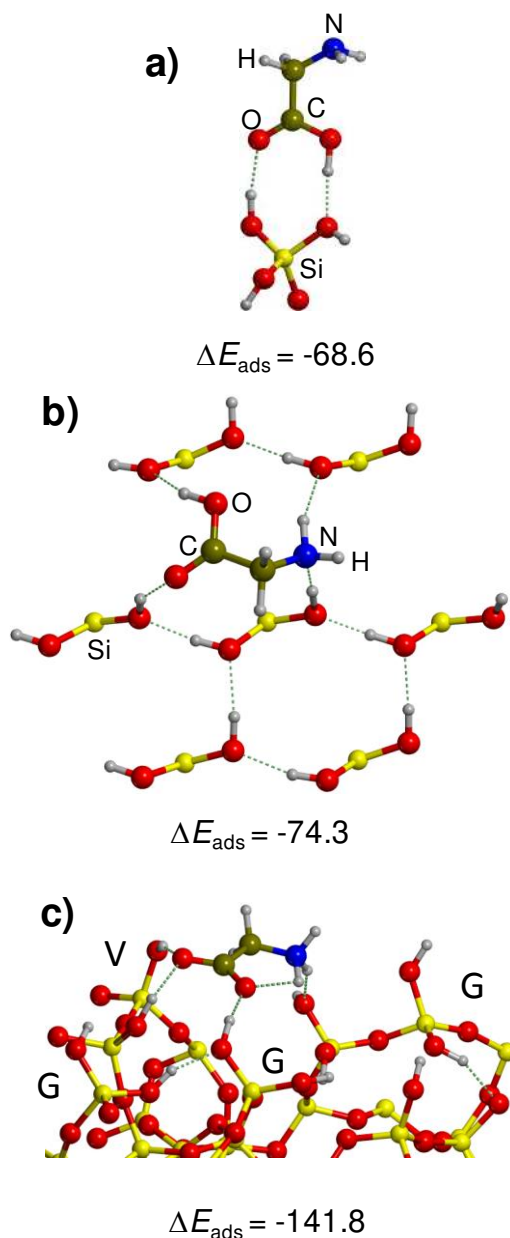
Figure 65. (a): Optimized structure and computed adsorption energy ( \Delta E_{\text{ads}} , in kJ mol -1 ) at B3LYP/6-31++G for Gly interacting with a minimal cluster ( \text{Si}(\text{OH})_4 ) model representing geminal silanol groups (drawn with data from Ref. 223 ). (b): Optimized structure and computed adsorption energy at PBE for Gly interacting with the hydroxylated (0001) \alpha -quartz surface (drawn with data from Ref. 651 ); (c): The dominant configuration obtained from several ab initio molecular dynamics simulations (PBE method and T= 300K) for Gly interacting with a silica surface model rich in geminal silanol groups (drawn with data from Ref. 641 ). The computed adsorption energy ( \Delta E_{\text{ads}} , in kJ mol -1 ) was obtained by performing a geometry optimization onto this configuration at the B3LYP/6-311++G(d,p) level. V and G refers to vicinal and geminal silanol groups, respectively.
