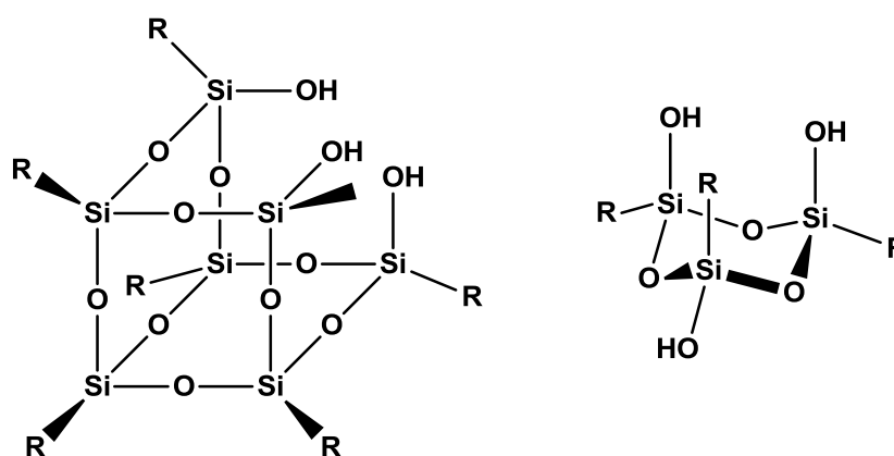
Figure 16. Left, a silsesquioxane bearing a group of 3 silanols in close vicinity. Right, a cyclotrisiloxane that could be used as a molecular mimic of a 3-ring.
