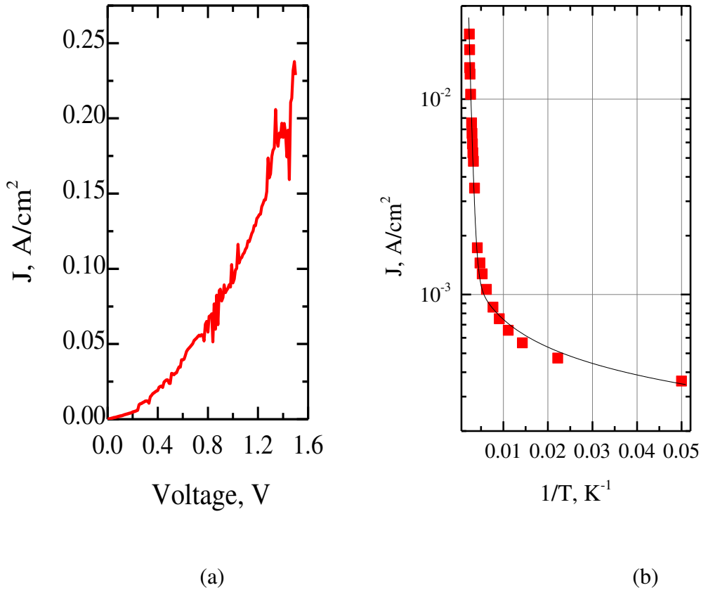
Figure 4.18 (a) I-V characteristics of NWs, (b) current density as function of temperature under reverse bias V=0.2V .
