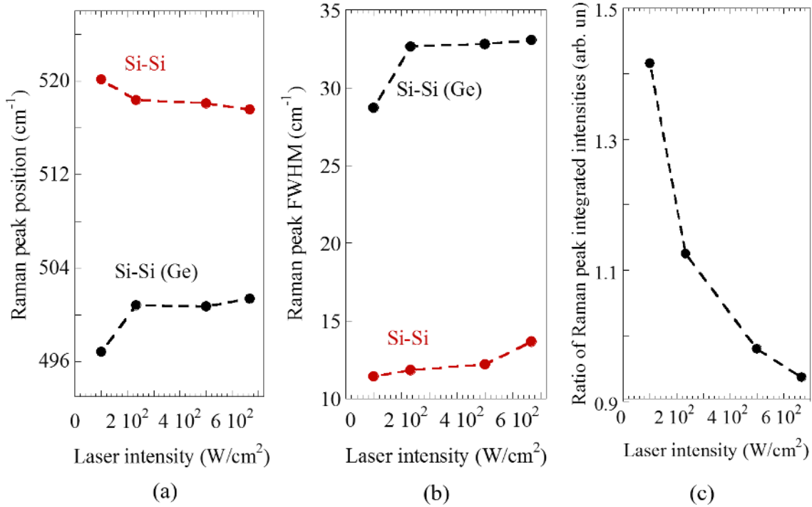
Figure 4.13 Comparison of the Raman signals associated with Si-Si and Si-Si(Ge) vibrations in Si/Ge NW HJs: (a) Raman peak position, (b) Raman peak FWHM, and (c) ratio of Si-Si to Si-Si(Ge) Raman peak integrated intensities as a function of the 458nm excitation intensity.
