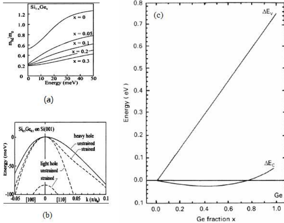
Figure 2.12 (a) Heavy hole effective mass density of states vs. energy at different x . (b) Valence band dispersion along [100] and [110] for \text{Si}_{0.5}\text{Ge}_{0.5} on Si(001). (schematic view). (c) Valence and conduction band offsets for strained \text{Si}_{1-x}\text{Ge}_x layers on (100) Si. Source: [101-103].
