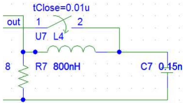
Figure 4.24 Spice simulation circuit biased in 0.5V DC coupling.
