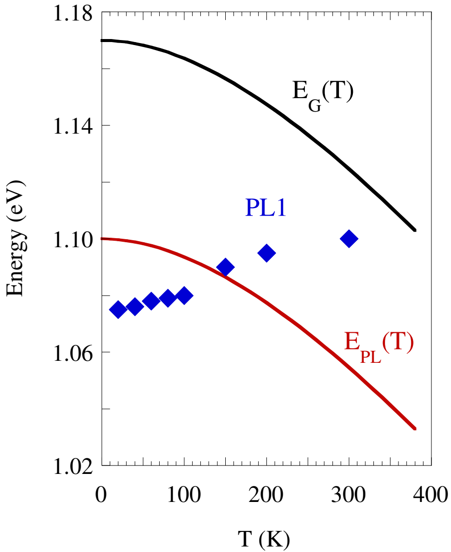
Figure 4.8 Temperature dependencies of c-Si energy gap, c-Si PL peak position, and PL1 peak position in Si/Ge W HJs. Source: [32].
