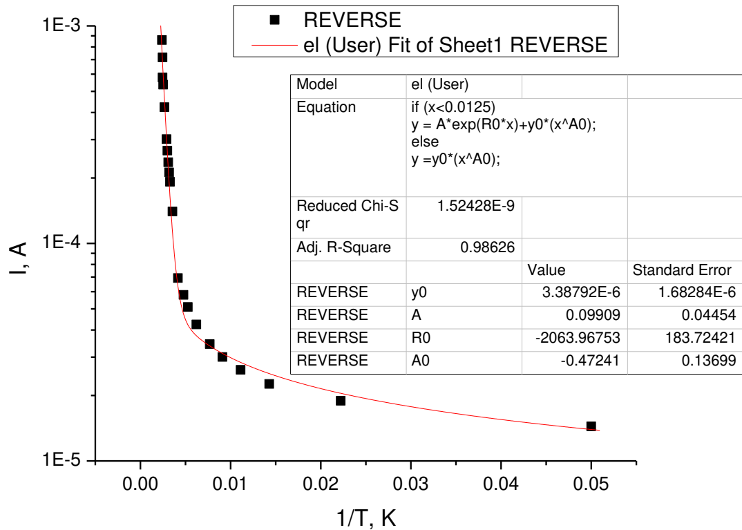
Figure 4.22 Current dependence on temperature at V= 0.2 V for reverse bias.
