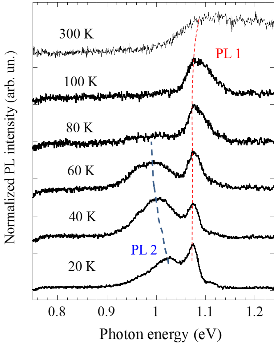
Figure 4.7 The PL spectra of the Si/Ge NW HJs at various (marked) temperatures. The major PL peak shifts with temperature increase are indicated by the dashed lines. Source: [32].
