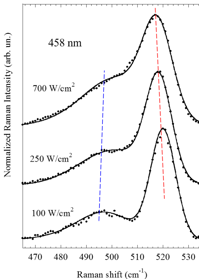
Figure 4.12 Background-corrected Raman spectra obtained under 458nm wavelength excitation and different (indicated) excitation intensities. Source: [32].
