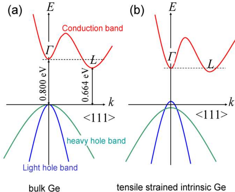
Figure 2.7 (a) A schematic view of band structure of bulk Ge, (b) tensile strained Ge with shifts towards direct bandgaps. Source: [83].
