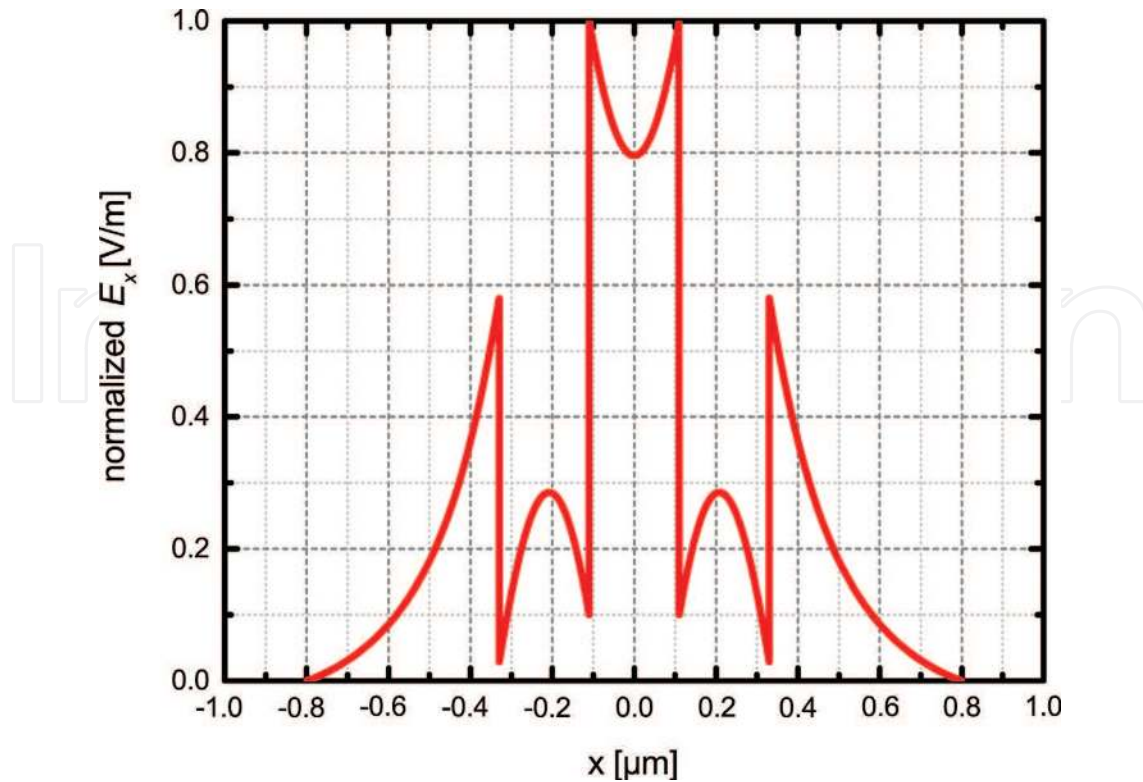
Figure 4. Calculated E_x field (normalized) for a slot waveguide structure with infinite height. Parameters: \lambda = 1550 nm, a = 110 nm, b = 220 nm, n_{slot} = n_{clad} = 1.44 , n_{si} = 3.48 .
