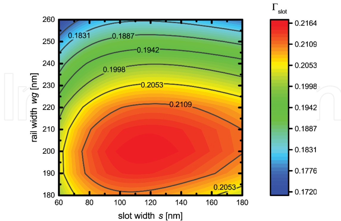
Figure 12. Calculated field confinement factor \Gamma_{slot} of an SOI slot waveguide for the slot region as a function of the slot width s and the rail width wg .
