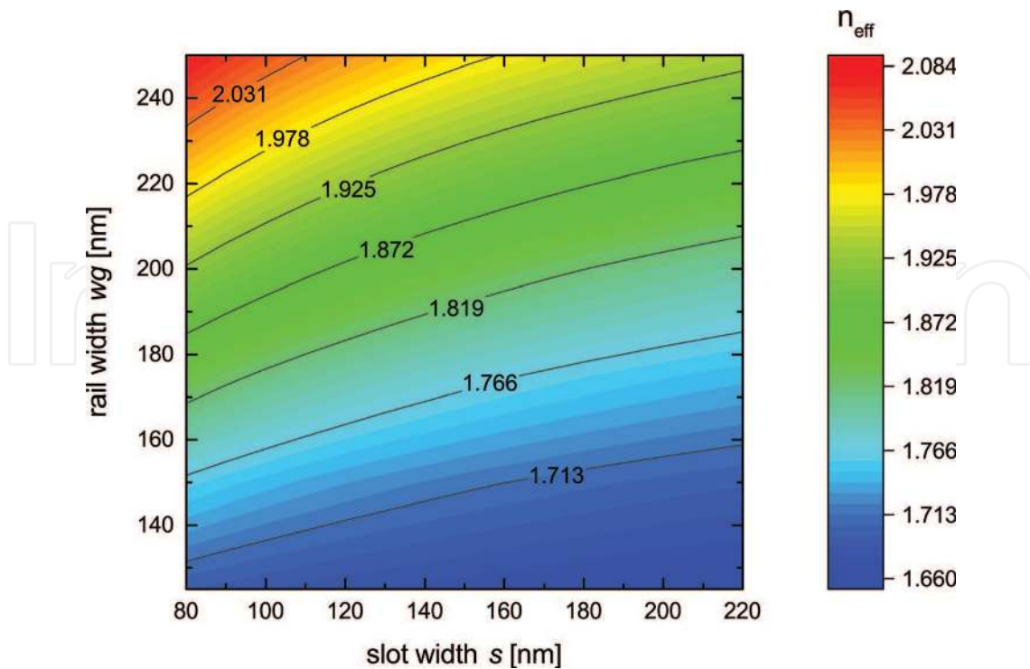
Figure 7. Calculated effective refractive indices n_{eff} of SOI slot waveguides as a function of the slot width s and the rail width wg .
