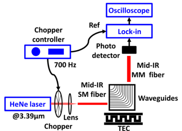
FIG. 3. Schematic of the experimental mid-IR setup used to characterize the silicon-on-nitride waveguides.
