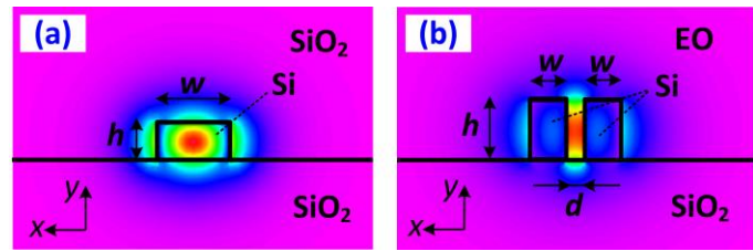
Figure 9: Schematic cross section of silicon photonic phase shifters. (a) Conventional phase shifter, exploiting refractive index changes due to free-carrier dispersion in the silicon (Si) waveguide core. (b) Slot-waveguide SOH phase shifter, exploiting the refractive index change in the organic electro-optic cladding (EO). In both structures, electric contacts have been omitted for simplicity.
