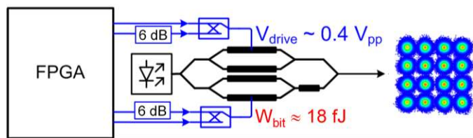
Figure 5: DAC-less amplifier-less generation of 16QAM signals by driving a highly efficient SOH IQ modulator from the binary CMOS outputs of a field-programmable gate array (FPGA) via a purely passive combiner network. The four-level drive signals for the in-phase (I) and quadrature (Q) arm of the modulator are generated by superimposing two binary signals, one of which is attenuated by a factor 2 in amplitude (6 dB). The resulting four-level signal has a peak-to-peak amplitude of 400 mV pp , and is sufficient to generate high-quality 16QAM signals at a symbol rate of 10 GBd and an energy consumption of only 18 fJ/bit [24].
