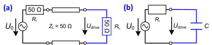
Figure 2: Equivalent-circuit models of EO modulators. (a) Impedance-matched travelling-wave device featuring an ohmic input load impedance of R_L = 50 \Omega , connected to a transmission line having a wave impedance Z_L = 50 \Omega and a signal source with an internal impedance of R_i = 50 \Omega . The modulator drive voltage is only half the internal source voltage, U_{\text{drive}} = U_0/2 . For estimating the energy consumption, the device is modeled by a single 50 \Omega resistor. (b) Underterminated lumped-element EO modulator represented by a capacitive load C . If the device is driven below its R_i C cut-off frequency, the drive voltage reaches a steady-state value which is equal to the open-circuit source voltage, U_{\text{drive}} = U_0 . The energy consumption is then dictated by the power dissipation in the resistor R_i during charging and discharging the capacitor. This power dissipation is independent of the exact value of R_i .
