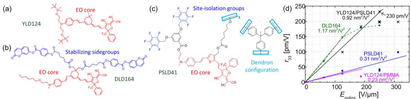
Figure 3: (a-c) Chemical structures of EO chromophores. The EO active cores are drawn in red. The materials DLD164 and PSLD41 consist of structurally engineered chromophores that enable high chromophore densities and a high degree of chromophore orientation during poling. Sidegroups that lead to matrix stabilization and enhancement of molecular orientation are marked in blue. (a) YLD124, used in guest-host systems (PMMA doped with 25 wt% YLD124) or in a binary-chromophore organic glass together with PSLD41 (25:75 wt%). (b) DLD164, used in pure form as a monolithic chromophore. (c) PSLD41, a dendritic molecule that combines three EO substructures, marked in light blue. (d) Measured poling efficiencies r_{33} / E_{\text{poling}} for the different organic cladding materials. We find extraordinarily high in-device electro-optic coefficients for DLD164 (190 pm/V) and for the YLD124/PSLD41 mixture (230 pm/V). (Figure adapted from [16])
