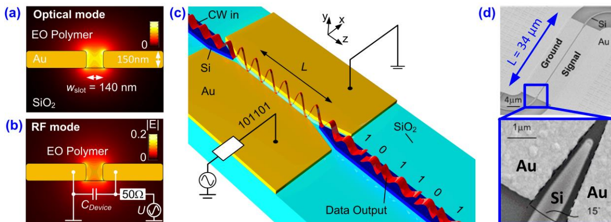
Figure 6: Plasmonic-organic hybrid (POH) phase modulator. (a) Optical mode: Light is guided as a surface plasmon polariton (SPP) mode of a metal slot waveguide. The slot is filled with an electro-optic (EO) polymer, and phase modulation is achieved by applying a modulating voltage to the metal sheets. (b) RF mode: The applied voltage drops entirely across the slot, leading to perfect overlap of the RF mode with the optical mode in the EO cladding. (c) POH modulator connected to dielectric SOI waveguides: Current plasmonic waveguides feature high propagation losses. It is therefore advantageous to embed the POH phase modulator into conventional silicon photonic circuitry that uses low-loss dielectric waveguides to transport light across the chip. (d) Mode converter between a photonic strip waveguide and a plasmonic slot waveguide made from gold (Au). The converter structures are approximately 3 \mu m long and feature power conversion efficiencies of more than 80 %. (Figure modified from [25])
