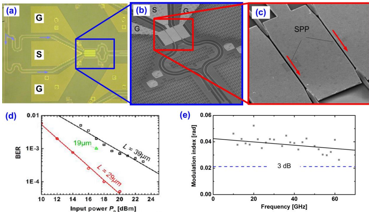
Figure 7: Experimental demonstration of a POH Mach-Zehnder Modulator (MZM). (a) The POH phase shifters are embedded into a Mach-Zehnder interferometer realized by conventional SOI strip waveguides. Electrical signals are fed to the device using a ground-signal-ground (GSG) electrode configuration. (b, c) Zoom-in of the POH phase shifters and the transitions between dielectric SOI waveguides and plasmonic slot waveguides. (d) Bit error ratio (BER) vs. optical input power P_0 into the POH MZM for different phase shifter lengths L . A phase shifter length of L = 29 \mu\text{m} leads to a compromise between the optical insertion loss and the modulation depth of the signal. (e) Frequency response of a 29 \mu\text{m} -long POH phase modulator. The graph depicts the modulation index as a function of the modulating frequency for a sinusoidal RF modulation signal delivered by a 50 \Omega generator with an available power of -10 \text{ dBm} . Grey dots indicate measured values, and the black line represents a linear fit to this data. The frequency response is essentially flat over the measurement range, except for a small frequency-dependent decay and some oscillations that we attribute to reflections from the POH modulator that acts as a capacitive load. To indicate the 3 dB limit, we include a dashed line at half the modulation index in the low-frequency limit. The device features a 3 dB bandwidth of significantly more than 60 GHz.
