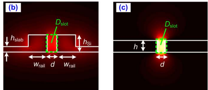
Figure 8: Field interaction of the optical mode with the EO cladding material. (a) Field interaction factor \Gamma_{\text{slot}} of the optical mode with the EO cladding material in the slot region D_{\text{slot}} as a function of slot width d for both POH and SOH waveguides at a wavelength of 1550 nm. The field interaction factor \Gamma_{\text{slot},x} as defined in Eq. (20) of the Appendix takes into account both the effects of spatial field overlap and of reduced group velocity. For the SOH device, the height of the silicon waveguides amounts to h_{\text{Si}} = 220 nm, and a value of w_{\text{rail}} = 240 nm was chosen for the width of the silicon rails, which represents approximately the optimum for a maximum field interaction factor \Gamma_{\text{slot},x} . In general, POH devices feature a 2.5 – 3.5 times larger field interaction factor than SOH devices due to the tight confinement of the plasmonic mode to the slot region and due to a reduced group velocity of the plasmonic slot mode. For POH devices, \Gamma_{\text{slot},x} decreases as the height h of the metal is reduced, since the mode field reaches further out of the slot region D_{\text{slot}} . Similarly, for SOH devices, \Gamma_{\text{slot}} decreases as the height h_{\text{slab}} of the silicon slabs is increased, since the optical mode field reaches out further into the slab region and the intensity within D_{\text{slot}} reduces. For the width of the silicon rails, the optimum value of w_{\text{rail}} \approx 240 nm represents a trade-off between strong field confinement in the silicon core for very wide rails and deep penetration of the mode field into the cladding for very narrow rails. (b) Cross section and mode field of an SOH phase shifter ( h_{\text{Si}} = 220 nm, w_{\text{rail}} = 240 nm, d = 120 nm, h_{\text{slab}} = 70 nm); (c) Cross section and mode field of a POH phase shifter ( h = 150 nm, d = 100 nm). The quasi-TE mode of the POH structure features a significantly stronger confinement to the slot region than its SOH counterpart.
