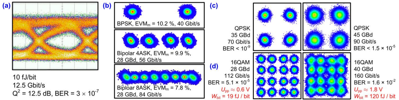
Figure 4: Experimental demonstration of high-performance SOH modulators. (a) Modulation at ultra-low energy consumption: When operating a short device with high electro-optic efficiency as a capacitive load, good signal quality can be obtained for modulation energies of a few femtojoule per bit [19], [20]. (b) Constellation diagrams for BPSK and bipolar ASK along with the corresponding error-vector magnitudes (EVM). BPSK transmission was found to be error-free. For the bipolar 4ASK (56 Gbit/s) and the bipolar 8ASK (84 Gbit/s), the measured BER amounted to 2 \times 10^{-6} and 9.7 \times 10^{-3} , respectively [17]. (c) Constellation diagrams of QPSK signals for symbol rates of 35 GBd and 45 GBd [22], [23]. No bit errors were detected within our record length of 62.5 \mu s for 35 GBd, and the error vector magnitude (EVM m ) indicate error-free signals with BER < 10^{-9} . At 45 GBd, the BER amounts to 1.5 \times 10^{-5} and is well below the threshold for hard-decision FEC with 7 % overhead. (d) Constellation diagrams of 16QAM-signals for symbol rates of 28 GBd and 40 GBd. For 28 GBd, the IQ modulator was operated with peak-to-peak voltages of U_{pp} = 0.6 V, leading to a power consumption of 19 fJ/bit and a BER of 5.1 \times 10^{-5} — well below the threshold for second-generation hard-decision FEC. For 40 GBd, the BER is still below the 2.4 \times 10^{-2} threshold for soft-decision FEC with 20 % overhead. (Figure adapted from [15])
