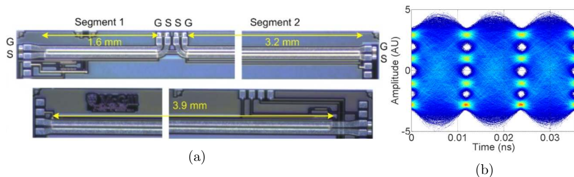
Figure 8: (a) Micrograph of a dual-segment (BWS) MZM (top) and a TW-MZM (bottom); (b) 84 Gbaud PAM-4 eye diagram of the dual-segment MZM. Figure reproduced from [48] © 2017 The Optical Society.
