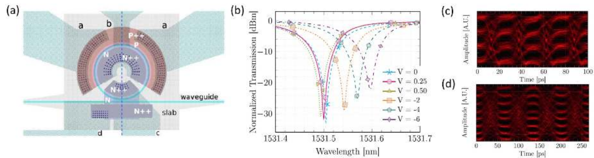
Figure 10: (a) Partial layout of the mask used for the fabrication of the device; (b) measured power transmission spectra in the vicinity of a resonance; (c) eye diagrams of the equalized PAM-4 at 80 Gbps; (d) eye diagrams of the equalized PAM-8 at 45 Gbps. The received power is 7 dBm. Figures reproduced from [15] © 2016 The Optical Society.
