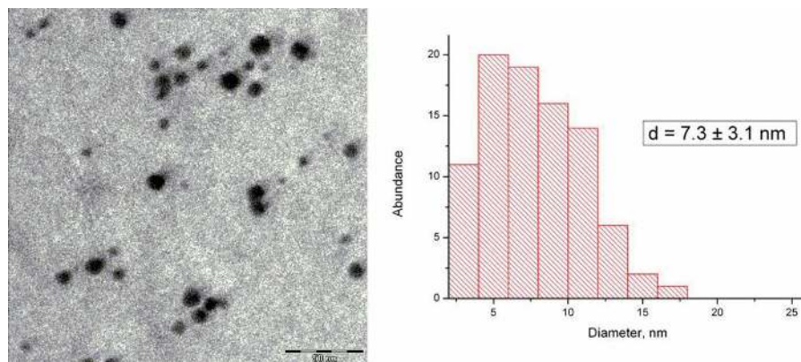
Fig. 1. A typical TEM micrograph (scale of 50 nm) and a size distribution histogram for silver nanoparticles prepared by the electrochemical method
