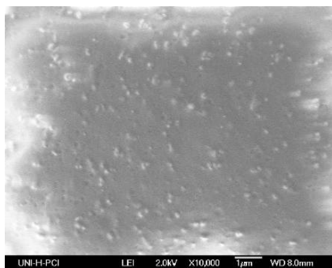
Fig. 2. A sample of water-soluble paint with immobilized silver nanoparticles
