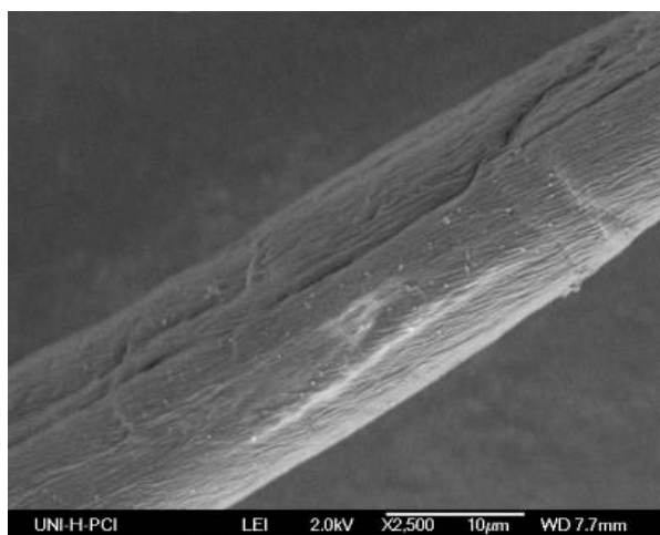
Fig. 4. A sample of 100% cotton with immobilized silver nanoparticles
