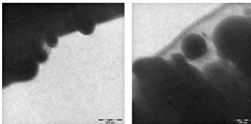
Fig. 5. A TEM image of silver nanoparticles on (left) and under (right) the surface of fibrous sorbent
