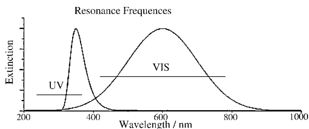
Fig. 5. Model of an UV/VIS spectrum with two extinction bands for two different polarisation directions of the two components of the electric field. Parallel to the short axis of the particles the resonance frequency is higher than parallel to the longer axis of the particles.
