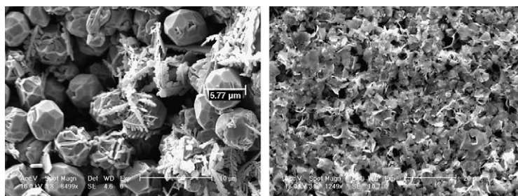
Fig. 3. Silver particles synthesised with addition of Tamol VS as stabilising agent and with addition of Lutensit A, ES as stabilising agent. Ascorbic acid was used as reductive agent.
