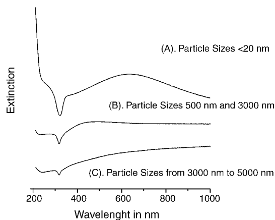
Fig. 4. UV/VIS measurements of silver particles: (a) silver particles with sizes, <20 nm, synthesised with iron ammonium citrate as reductant; (b) silver particles with 500 and 3000 nm in diameter, synthesised with ascorbic acid as reductant and PVP K 25 as stabilising agent; and (c) silver particles with sizes in the range from 3000 to 5000 nm in diameter, synthesised with ascorbic acid as reductant and Tamol VS as stabilising agent.
