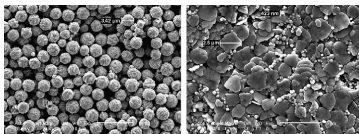
Fig. 2. Silver particles synthesised with addition of Plurafac LF 221 as stabilising agent (left) and with addition of PVP as stabilising agent (right). Ascorbic acid was used as reductive agent.
