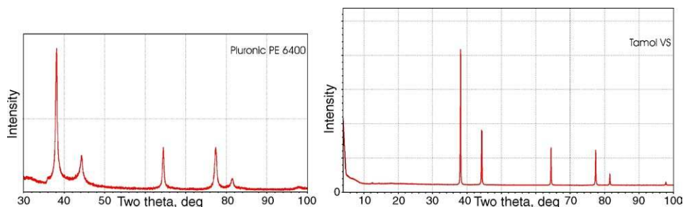
Fig. 1. X-ray patterns characteristic for a cubic system of crystalline metallic silver exhibit diversity in peak intensity and width.
