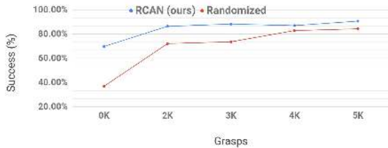
Figure 4: A graph showing how the performance of RCAN and directly learning a policy on domain randomization varies with the number of real world on-policy grasps.
