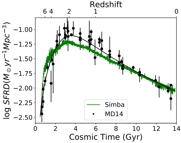
Figure 7. Star formation rate density evolution versus age of the Universe in SIMBA (curve), compared to the observational compilation of Madau & Dickinson (2014) (black points and best-fit line).
