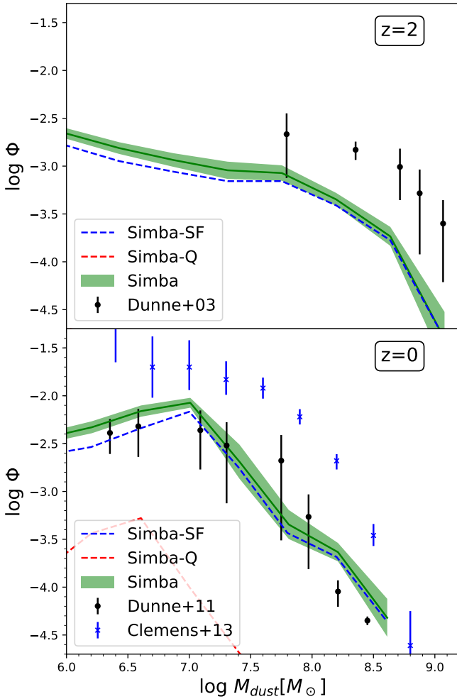
Figure 14. Dust mass function from SIMBA at z = 0 , shown as the green shaded region. DMF is split into star-forming and quenched samples, shown as blue and red dashed lines, respectively. Observations are shown from Dunne et al. (2011) and Clemens et al. (2013); differences owe to assumptions regarding inferring dust mass from far-IR flux. SIMBA reproduces the observed shape of the DMF, and is in the range of observed amplitudes, modulo systematic uncertainties.
