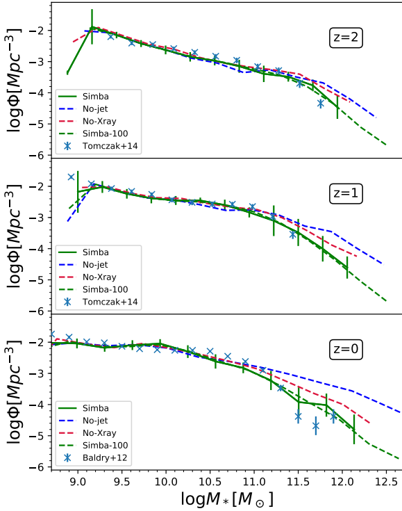
Figure 17. Stellar mass function evolution from z = 2 \rightarrow 0 in 50h^{-1}\text{Mpc} , 512^3 test runs with different AGN feedback variants: Original SIMBA (green solid), Jet and X-ray feedback both turned off (No-jet; blue dashed), only X-ray feedback turned off (No-Xray; red dashed). For comparison we show the main 100h^{-1}\text{Mpc} SIMBA run (green dashed) reproduced from Figure 4, as well as selected observations as indicated. Turning on just the jet feedback (No-Xray) results in a substantial truncation of the GSMF that does not occur without jets (No-jet).
