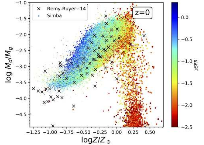
Figure 15. Dust to gas ratio as a function of gas-phase metallicity at z = 0 in SIMBA galaxies, colour-coded by specific SFR. Observations are shown as crosses from Rémy-Ruyer et al. (2014). SIMBA reproduces the observed trend and amplitude in dust-to-gas ratios.
