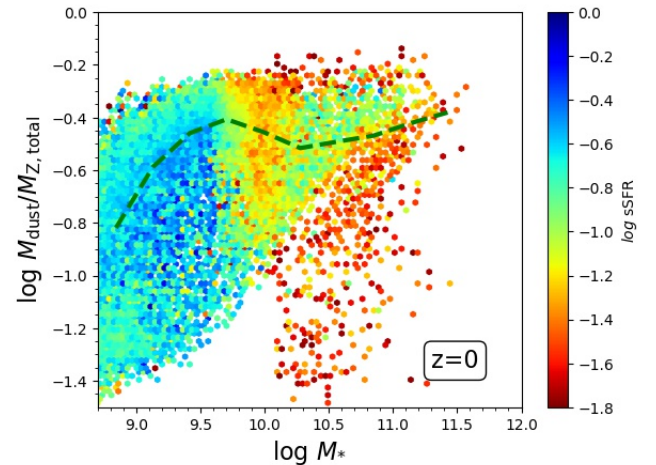
Figure 16. Metal mass fraction locked in dust, as a function of M_* , for star-forming galaxies in SIMBA. Plot is colour-coded by the mean sSFR within each hexbin. Except for the smallest galaxies, typically one-third of the metals are locked in dust.
