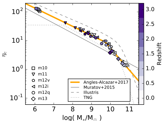
Figure 1. Mass loading factor \eta versus stellar mass M_* from a suite of FIRE simulations analysed via particle tracking in Anglés-Alcázar et al. (2017b). The points show values measured at various redshifts, while the orange line is the best-fit relation. The gray solid line shows the Muratov et al. (2015) scaling and the dashed and dotted gray lines show the mass loading factors used in the Illustris and Illustris-TNG simulations ( \eta(M_{\text{halo}}) fitting functions from Pillepich et al. 2018, converted to \eta(M_*) using the M_*-M_{\text{halo}} relation of Moster et al. 2013).
