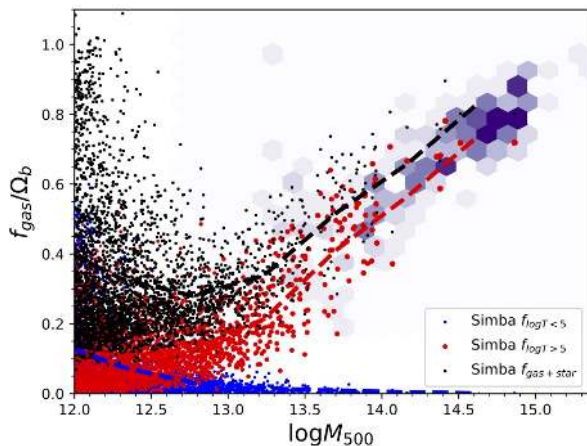
Figure 12. Gas fractions as a function of M_{500} at z = 0 . Black points show the total baryon fraction within the halo, and red and blue points show the gas fractions subdivided at 10^5\text{K} . Purple hexbins show an observational compilation of hot gas fractions from McCarthy et al. (2017), to be compared to the red points. SIMBA does a reasonable job of reproducing the observed trend of hot gas fraction with M_{500} , which has been difficult for previous simulations to achieve without tuning.
