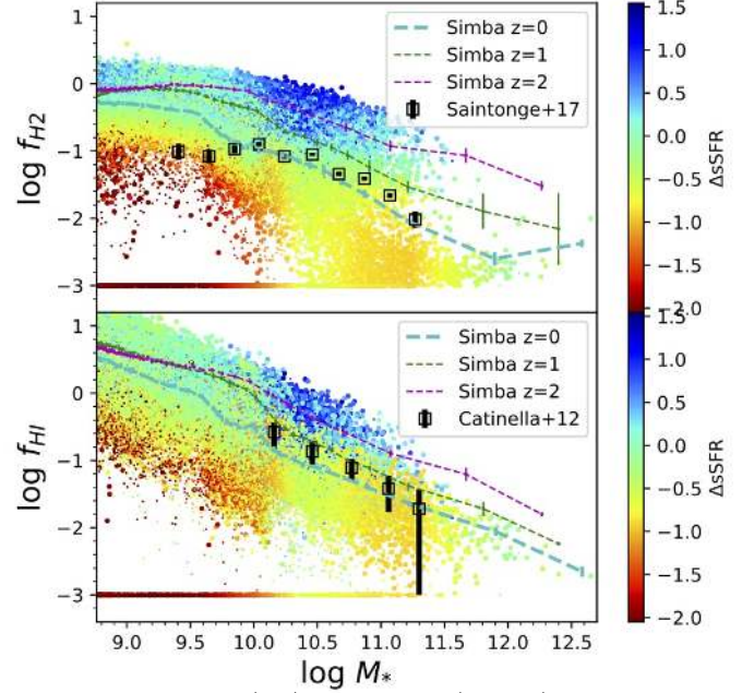
Figure 8. Molecular (top) and neutral (bottom) gas fractions M_{H_2}/M_* and M_{HI}/M_* as a function of M_* . The points show z = 0 values from SIMBA colour-coded by the deviation in sSFR from the star-forming main sequence – bluer points have higher-than typical SFR, redder have lower. A running median at z = 0 is shown as the cyan dashed line. For comparison we show the running medians at z = 1, 2 (green, magenta lines). Observations of f_{H_2} from xCOLDGASS (Saintonge et al. 2017) are shown in the top panel, and observations of f_{HI} from GASS (Catinella et al. 2012) are shown in the bottom panel. SIMBA predicts gas fraction scalings in good agreement with data, and predicts a small but significant amount of gas even in the most massive quenched systems.
