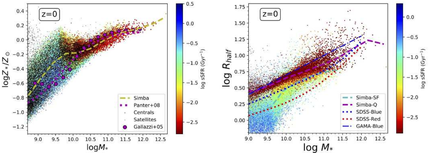
Figure 11. R -band 2-D projected half-light radii of SIMBA galaxies at z = 0 , as a function of M_* . Points are colour-coded by sSFR. We fit median relations to the red and blue sub-samples, delineated by 10^{-1.8} \text{ Gyr}^{-1} , as the cyan and magenta dashed lines, respectively. Observational relations are shown from Zhang & Yang (2017) from SDSS, split into red and blue galaxies. SIMBA broadly reproduces the sizes of star-forming galaxies, but fails to show the observed trend that quiescent galaxies have a much steeper slope and are much more compact at low masses.
