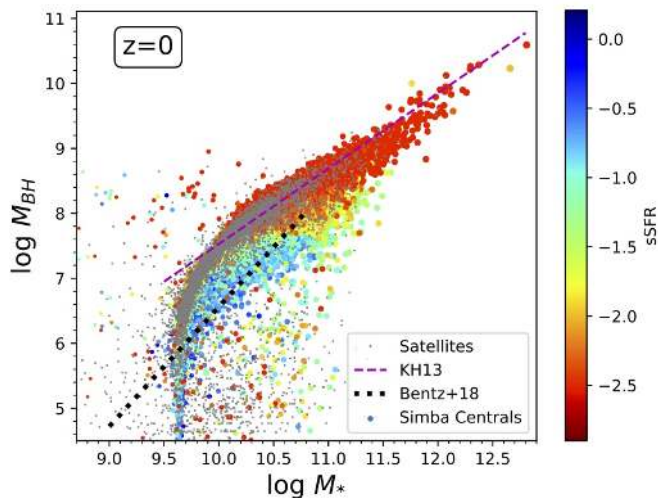
Figure 13. M_{\text{BH}} - M_* relation at z = 0 in SIMBA. Points show galaxies, with centrals colour-coded by specific SFR, and satellites as the grey points. Observations are shown from Kormendy & Ho (2013) for comparison with bulge-dominated (redder) systems, while Bentz & Manne-Nicholas (2018) shows the relationship more appropriate for spiral star-forming systems at lower M_* . SIMBA broadly reproduces these observed relations in its appropriate galaxy populations.
