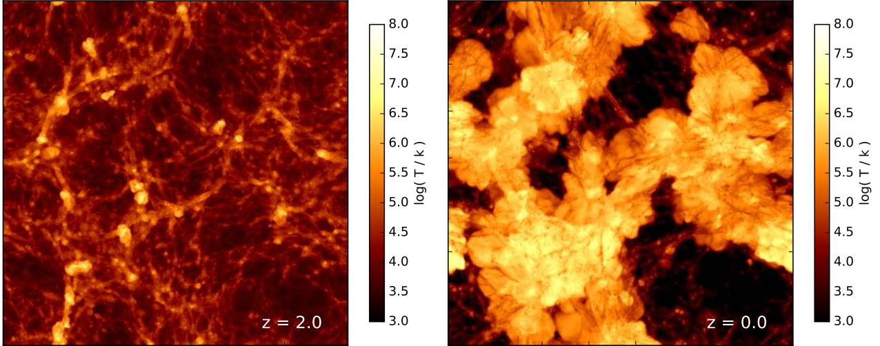
Figure 2. Temperature map projected through a random 10 Mpc/h slice from a 50 Mpc/h SIMBA volume, at z = 2 (left) and z = 0 (right). At z = 2 , warm-hot gas traces large-scale filaments, with energetic bipolar outflows owing to jets evident from the nodes where the most massive galaxies and black holes reside. At z = 0 , high-speed AGN outflows have shocked the IGM gas throughout much of this volume to well beyond the virial radii of halos, with cooler dense filamentary structures penetrating the hot gas.
