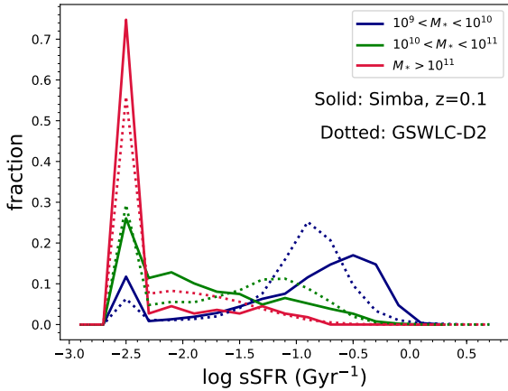
Figure 6. Histogram of sSFR in three bins of stellar mass. Solid lines show the results for SIMBA at z = 0.1 , while dotted lines show z \sim 0.1 observations from GSWLC-D2. All galaxies with sSFR < 10^{-2.5} \text{ Gyr}^{-1} are placed in the lowestmost bin. There is good agreement, particularly in the quenched fractions in more massive galaxies, though SIMBA produces somewhat too high sSFRs at low- M_* .
