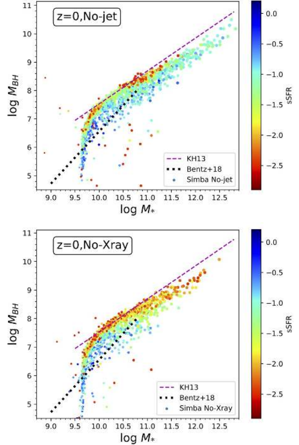
Figure 18. M_{\text{BH}} - M_* relations in test simulations with jet and X-ray black hole feedback turned off (No-jet, top panel), and jets on but X-ray feedback turned off (No-Xray, bottom). By comparing to Figure 13, the jet feedback is seen to enact most of the quenching, but the X-ray feedback is important for fully quenching the most massive galaxies.
