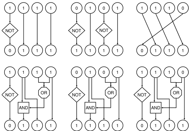
Figure 2: Illustration of RELEVANCE under the Boolean circuit formalization. The three pairs of objects (1111, 0111) , (0101, 1111) , and (1110, 0111) can be each be transformed by one of the three circuits shown at the top. No one of these circuits can transform these three pairs of objects and pair (0011, 1001) in Figure 1, but the circuit at the bottom is capable of transforming them all. If all these circuits were psychologically possible, i.e. in \mathcal{T} , then in our formalization of RELEVANCE the circuit at the bottom would be considered relevant for the set of pairs X = \{(1111, 0111), (0101, 1111), (1110, 0111), (0011, 1001)\} , whereas the other circuits would not be.
